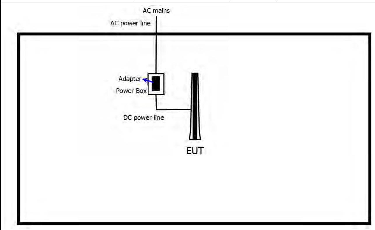
Test Setup Diagram - Radiated Test(above 1GHz)
