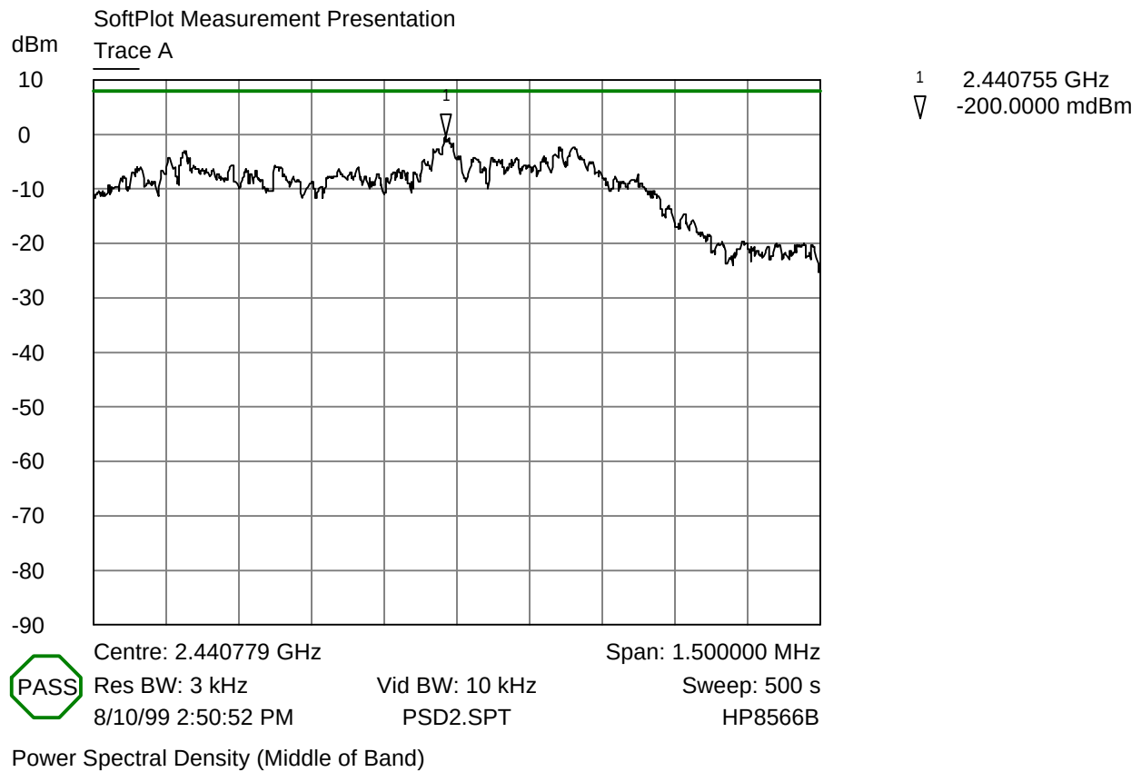
Power Spectral Density Plot - Handset (Middle Channel)
