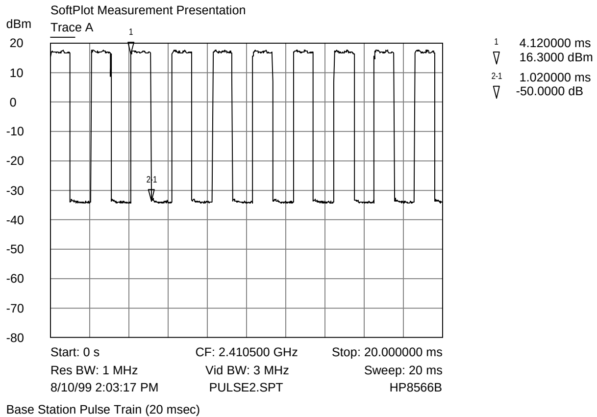
Pulse Train Plot - Base Station (20 msec)
