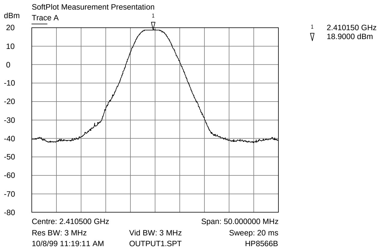
Peak Output Power Plot – Base Station (Low Channel)
