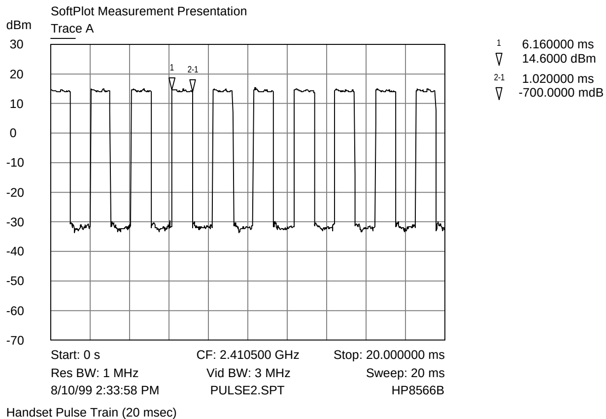
Pulse Train Plot - Handset (20 msec)
