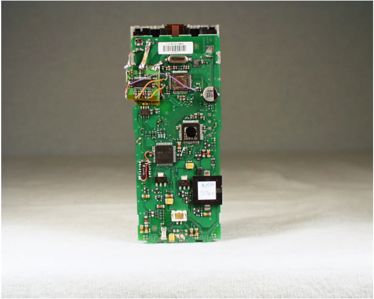
Inside View - Side B - Handset
