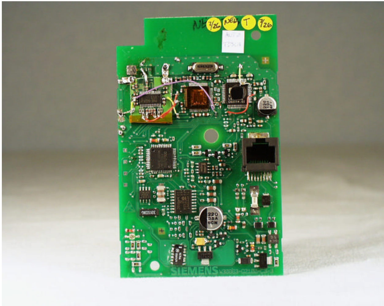
Inside View - Side A - Base Station
