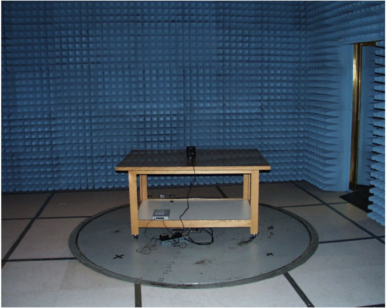
Back view of worst case radiated emissions (Base Station)
