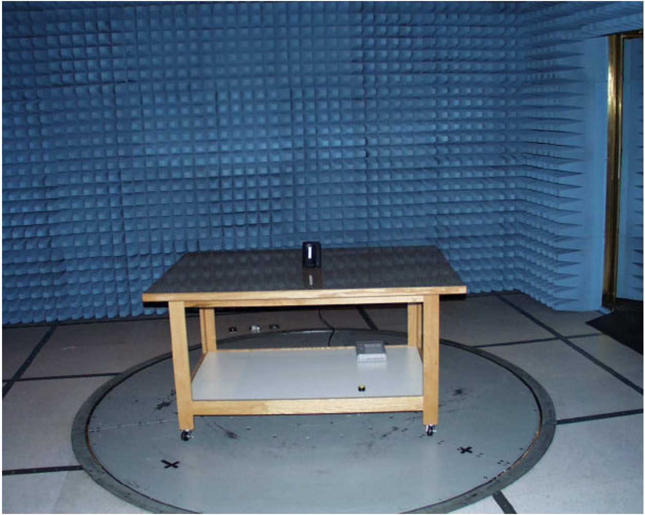
Front view of worst case radiated emissions (Base Station)
