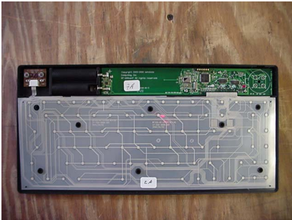
Circuit Top with Keypad Contacts
