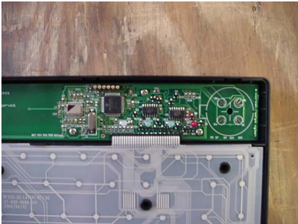
Circuit Top Right Close Up
