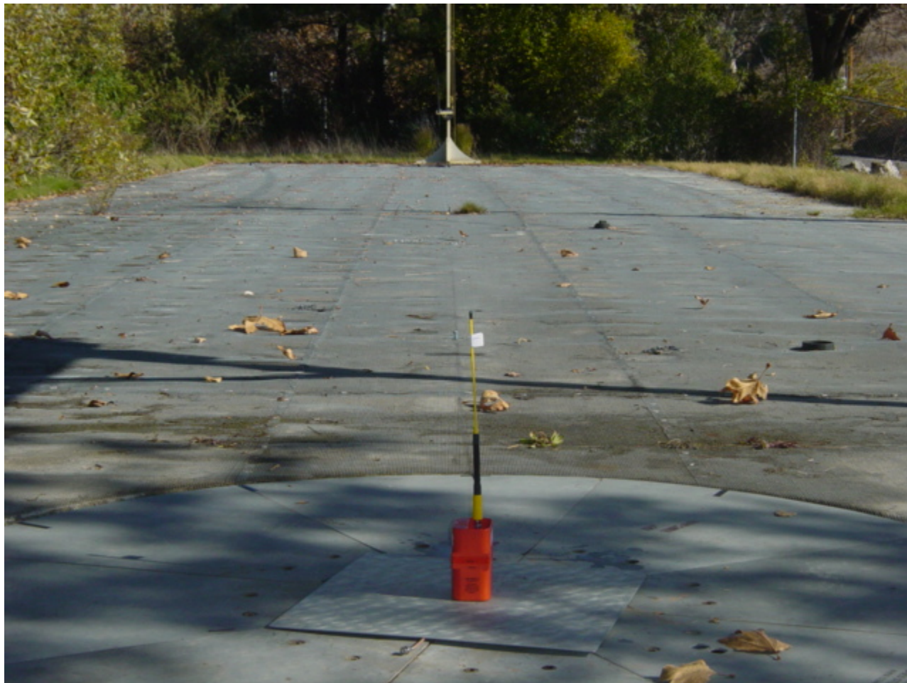
PHOTOGRAPH OF THE TEST SETUP FOR RADIO FREQUENCY RADIATED INTERFERENCE
