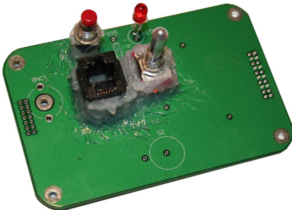
Switch PCB assembly bottom side
