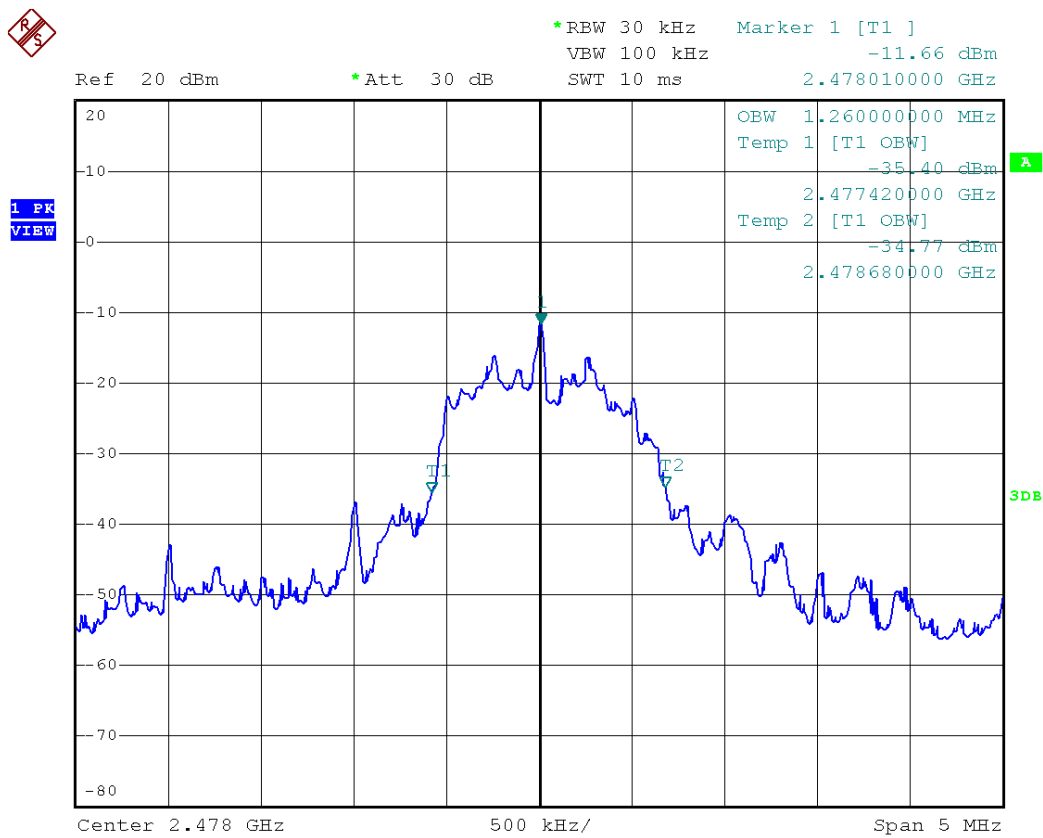
Figure 23- 99% Bandwidth Measurement (fc=2478MHz)
