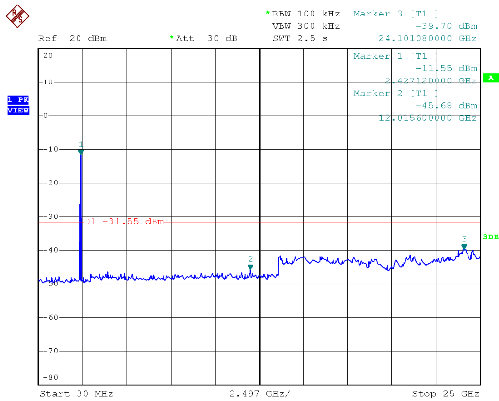
Figure 15 Conducted Spurious Emissions, mid channel
