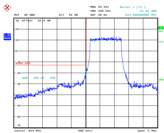
Figure 4-41a: Band 5 Low Channel Mask, 1.4MHz BW, RB=6
