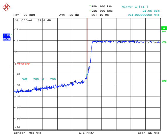
Figure 6-25a: Band 17 Low Channel Mask, 10MHz BW, RB=50
