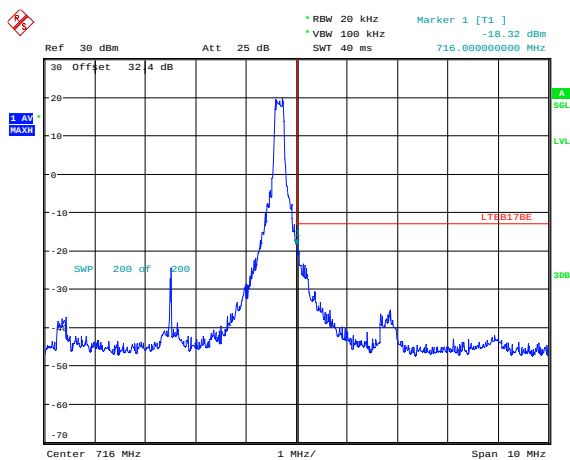
Figure 6-32a: Band 17 High Channel Mask, 5MHz BW, RB=1
