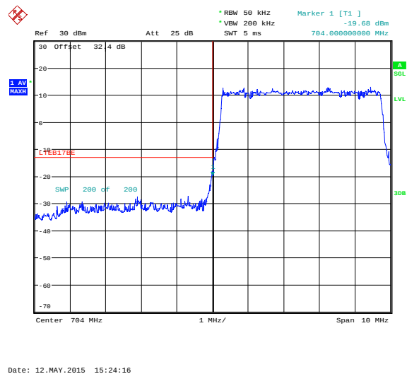
Figure 6-29a: Band 17 Low Channel Mask, 5MHz BW, RB=25
