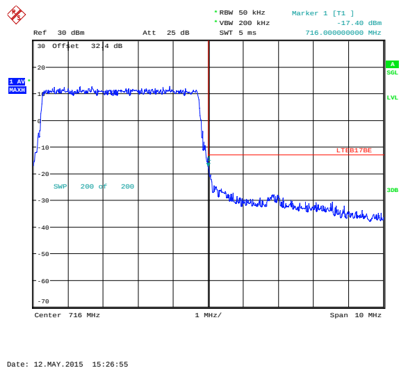
Figure 6-30a: Band 17 High Channel Mask, 5MHz BW, RB=25
