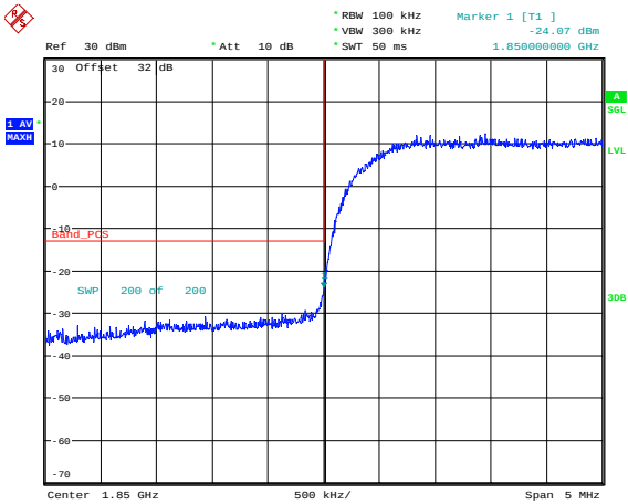
Figure 2-52a: Band II, HSUPA Low Channel Mask
