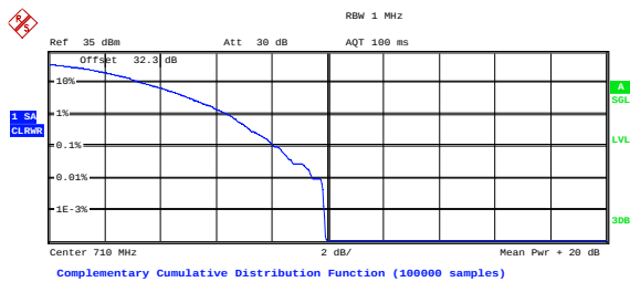
Figure 6-34a: Band 17 Middle Channel PAR, 10MHz BW, RB=50
