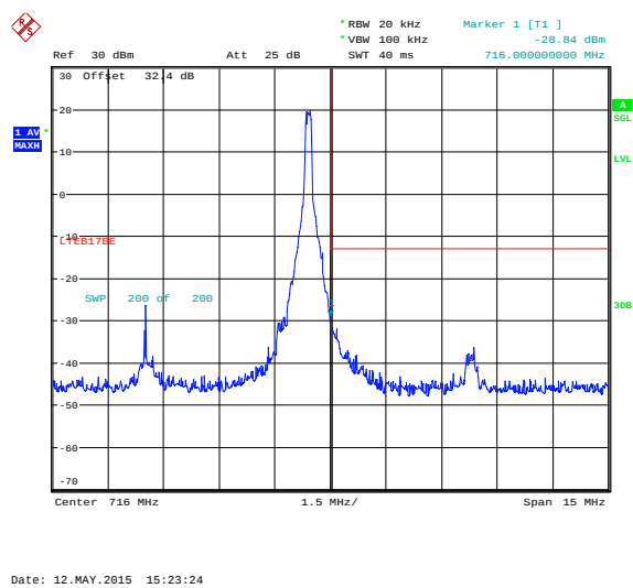
Figure 6-28a: Band 17 High Channel Mask,10MHz BW, RB=1
