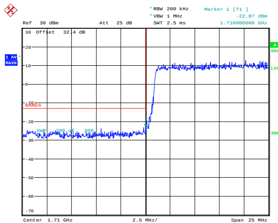
Figure 5-37a: Band 4 Low Channel Mask, 20MHz BW, RB=100
