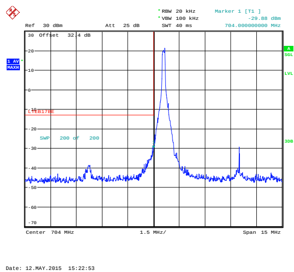
Figure 6-27a: Band 17 Low Channel Mask, 10MHz BW, RB=1
