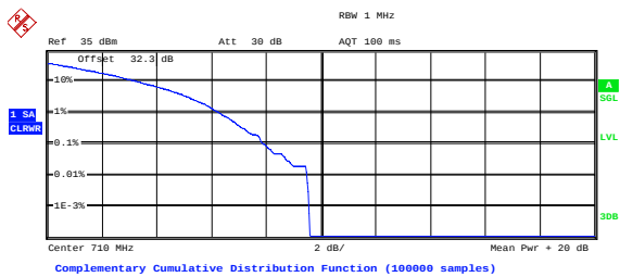
Figure 6-33a: Band 17 Mid Channel PAR, 10MHz BW, RB=25
