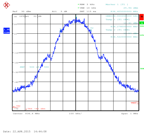
Figure 1-16a: Occupied Bandwidth, GSM850 band Middle Channel in GSM mode
