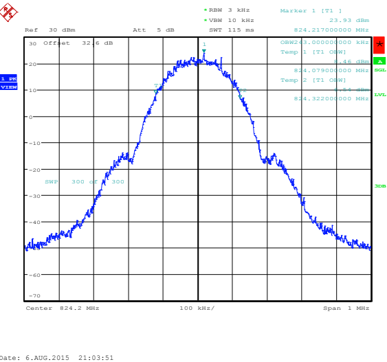
Figure 1-29a: Occupied Bandwidth, GSM850 Band, Low Channel in EDGE mode
