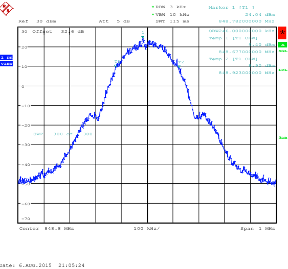
Figure 1-31a: Occupied Bandwidth, GSM850 band, High Channel in EDGE mode
