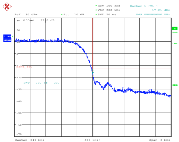
Figure 2-25a: Band V , HSUPA High Channel Mask
