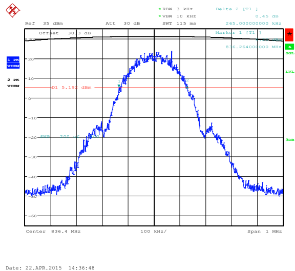
Figure 1-15a: -26dBc bandwidth, GSM850 band Middle Channel in GSM mode
