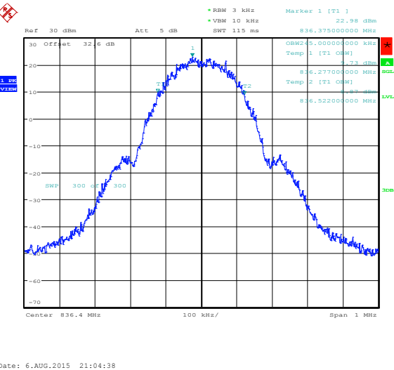
Figure 1-30a: Occupied Bandwidth, GSM850 Band, Middle Channel in EDGE mode
