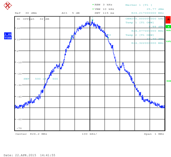
Figure 1-14a: Occupied Bandwidth, GSM850 band Low Channel in GSM mode
