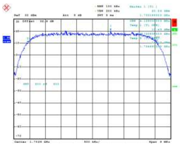
Figure 2-8b: Occupied Bandwidth, Band IV Middle Channel
