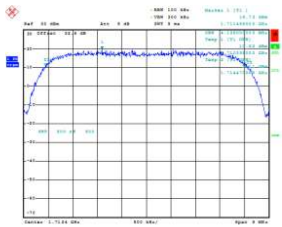
Figure 2-7b: Occupied Bandwidth, Band IV Low Channel
