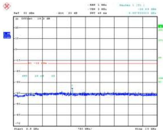
Figure 3-8a: Band 2, Spurious Conducted Emissions, Low channel, 10MHz BW (RB= 1)
