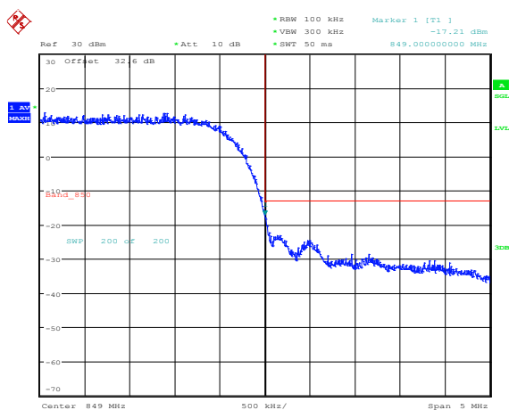
Figure 2-25a: Band V , HSPA High Channel Mask
