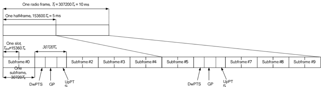
Figure 1: Frame structure type 2 (for 5ms switch-point periodicity)
