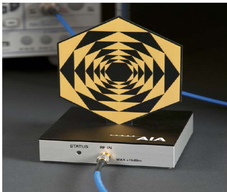
Figure 5.4-1: Audio Interference Analyzer
