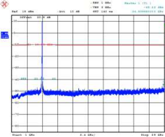
Figure 8-137: Spurious RF Conducted Emissions Primary, 802.11ac, Channel 149, MCS0 Mbps
