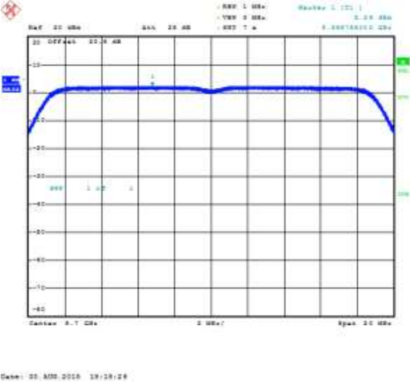
Figure 8-77: Peak Power Spectral Density MIMO Secondary, 802.11ac, Channel 140, MCS0 Mbps
