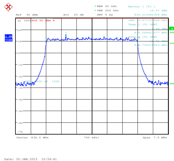
Figure 5-23a: Occupied Bandwidth, Band 5 Middle Channel, 5MHz BW, RB=25
