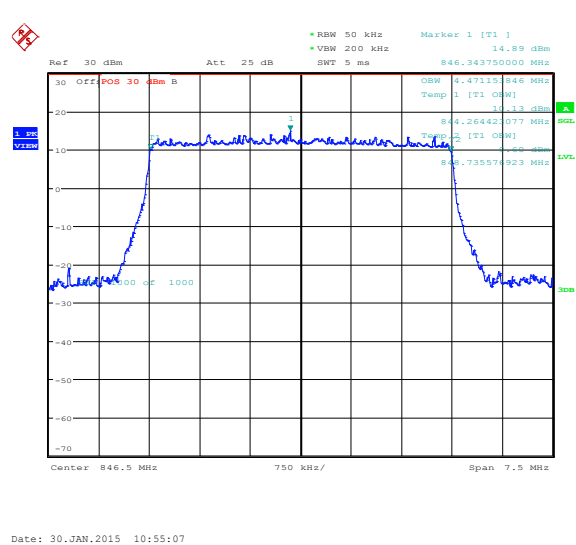
Figure 5-24a: Occupied Bandwidth, Band 5 High Channel, 5MHz BW, RB=25
