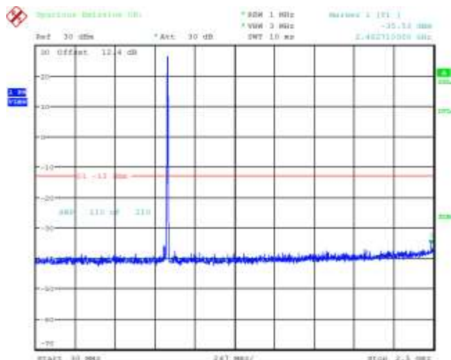
Figure 5-17a: Band 5, Spurious Conducted Emissions, High channel, 1.4MHz BW (RB= 6)
