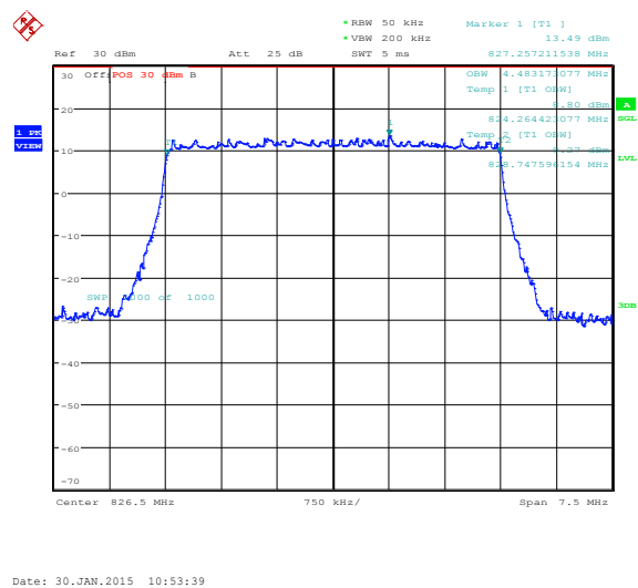
Figure 5-22a: Occupied Bandwidth, Band 5 Low Channel, 5MHz BW, RB=25
