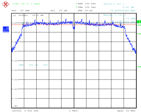
Figure 4-41: 6 dB Bandwidth
