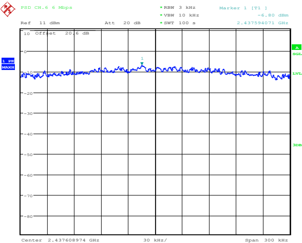
Figure 4-20: Peak Power Spectral Density 802.11g, Channel 6, 6 Mbps
