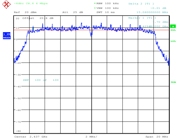
Figure 4-38: 6 dB Bandwidth
