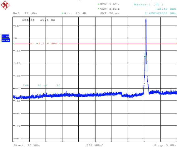
Figure 4-29: Spurious Conducted RF Emissions 802.11g, Channel 6, 6 Mbps
