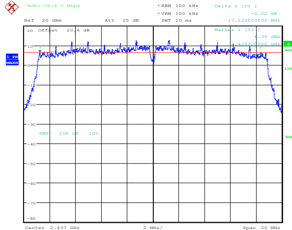
Figure 4-39: 6 dB Bandwidth
