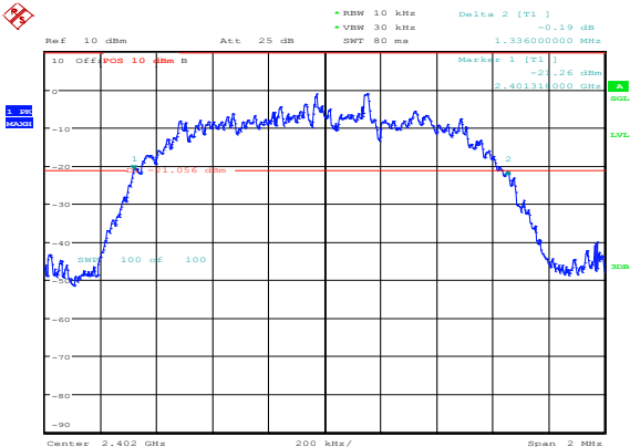
Figure 3-7: 20 dB Bandwidth Single freq., Static PBRs, 3-DH5
