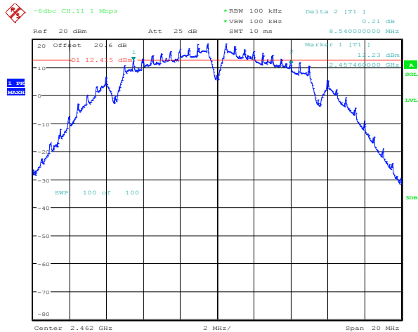
Figure 4-40: 6 dB Bandwidth
