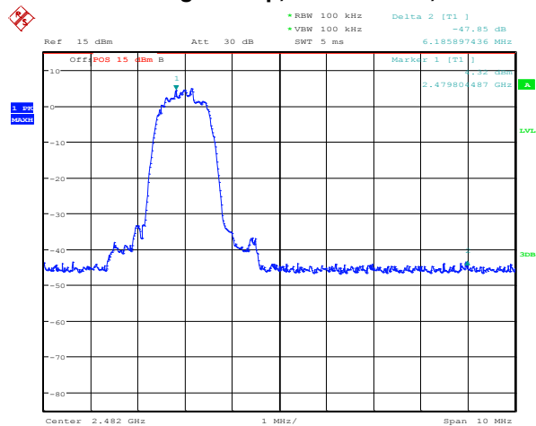
Figure 3-35: Band Edge Compliance Single Freq., Static PBRS, 3-DH5
