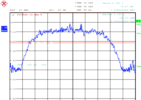
Figure 3-9: 20 dB Bandwidth Single freq., Static PBRs, 3-DH5
