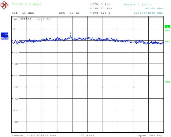
Figure 4-53: Peak Power Spectral Density 802.11g, Channel 6, 6 Mbps
