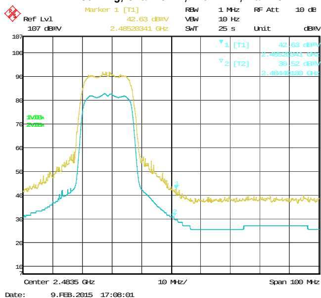
Figure 2-23: Band-Edge Compliance of RF Radiated Emission
