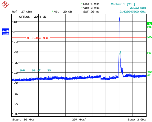
Figure 4-36: Spurious Conducted RF Emissions 802.11b, Channel 11, 1 Mbps
