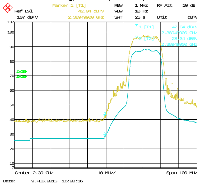
Figure 2-24: Band-Edge Compliance of RF Radiated Emission
