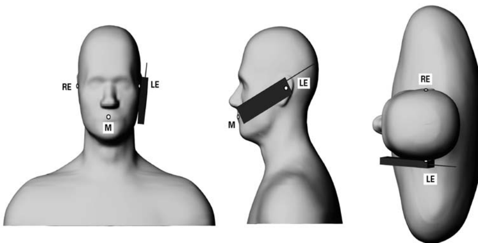
Figure 8.2.1-3 Phone position 1, “cheek” or “touch” position. The reference points for the right ear (RE), left ear (LE) and mouth (M), which define the reference plane for phone positioning, are indicated. The shoulders are shown for illustration purposes only.
