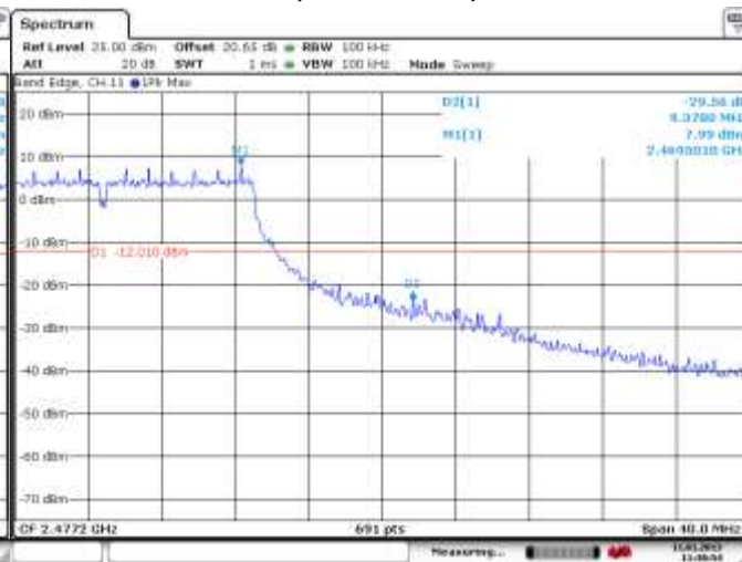
Figure 5-15: Band Edge Compliance 802.11n, Channel 11, MCS 0
