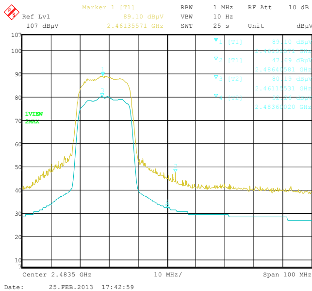
Figure 2-27: Band-Edge Compliance of RF Radiated Emission 802.11n, Channel 11, 2462 MHz, Max Pol: V, Detector: PK
