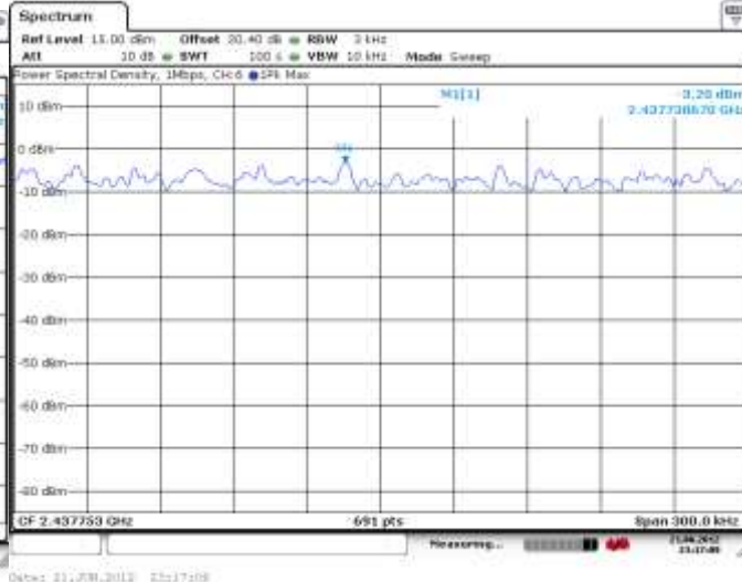
Figure 5-17: Peak Power Spectral Density 802.11b, Channel 6, 1 Mbps
