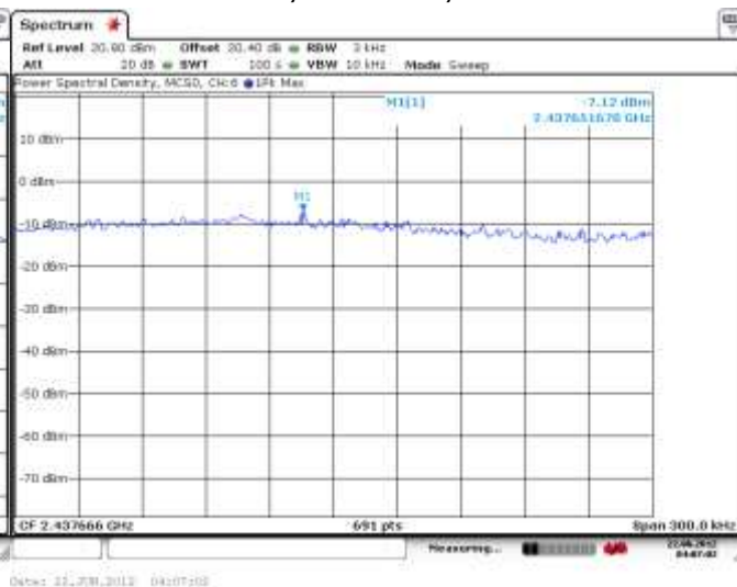
Figure 5-23: Peak Power Spectral Density 802.11n, Channel 6, MCS 0
