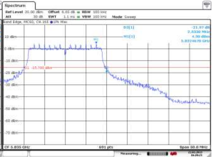
Figure 6-15: Band Edge Compliance 802.11a, Channel 165, 6 Mbps
