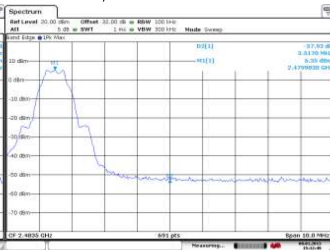
Figure 4-63: Band Edge Compliance LE, Channel 39
