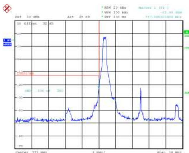
Figure 3-18a: Band 13 Low Channel Mask, 5MHz BW, RB=1
