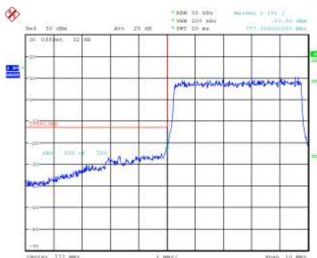
Figure 3-19a: Band 13 Low Channel Mask, 5MHz BW, RB=25
