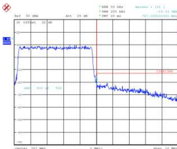
Figure 3-21a: Band 13 High Channel Mask, 5MHz BW, RB=25
