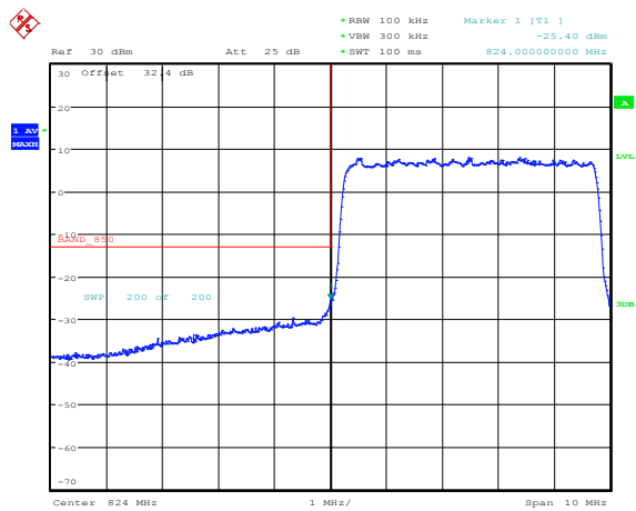
Figure 4-39a: Band 5 Low Channel Mask, 5MHz BW, RB=25
