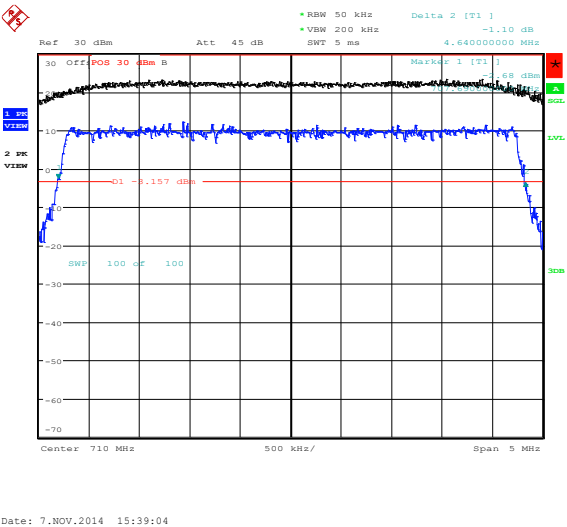
Figure 6-23a: -26 dBc Bandwidth, Band 17 Middle Channel, 5MHz BW, RB=25
