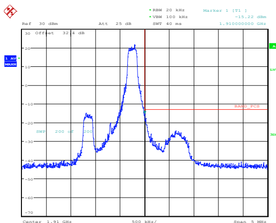
Figure 3-36a: Band 2 High Channel Mask, 1.4MHz BW, RB = 1
