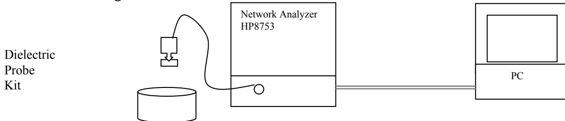
Figure 6.2.2-1 Test configuration
