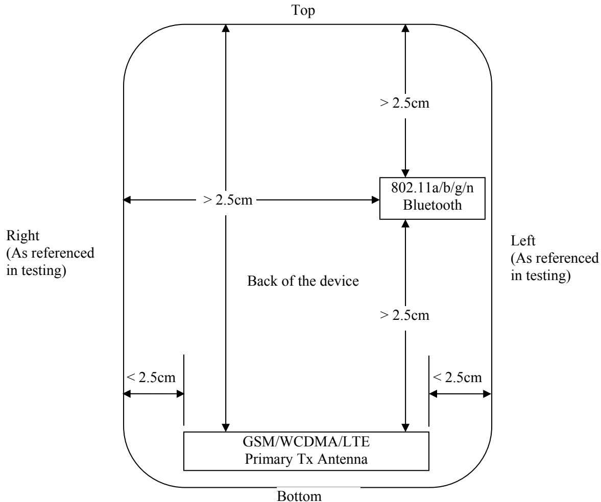
Figure 1.8.3-1 Identification of all sides for SAR Testing.
