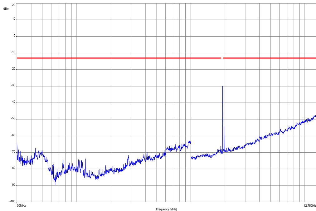
Plot 5: Channel 810 (30 MHz – 12.75 GHz), GSM
