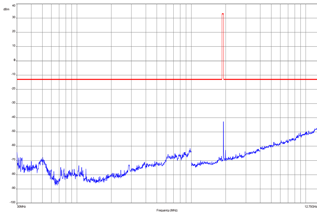
Plot 5: Channel 9538 (30 MHz – 12.75 GHz), voice
