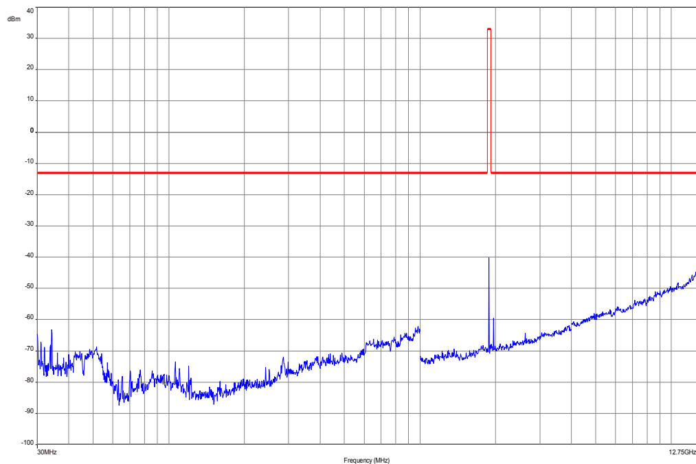
Plot 3: Channel 9400 (30 MHz – 12.75 GHz), voice
