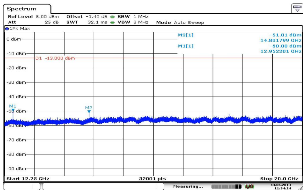
Plot 2: Channel 512 (12 GHz - 20 GHz), GSM
