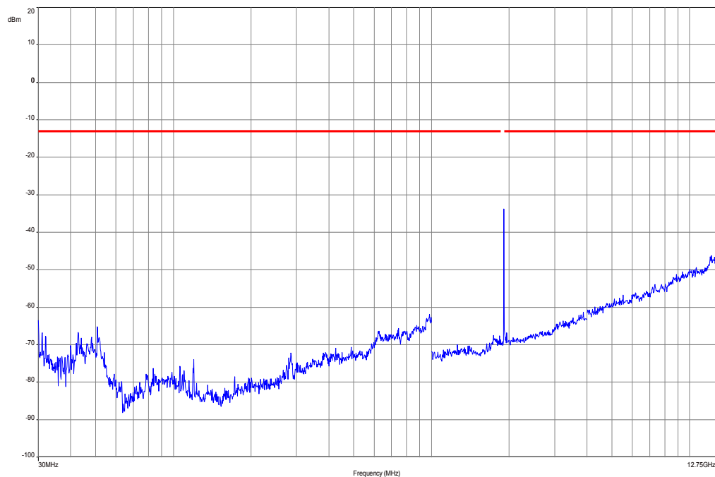
Plot 13: Channel 810 (30 MHz – 12.75 GHz), EDGE
