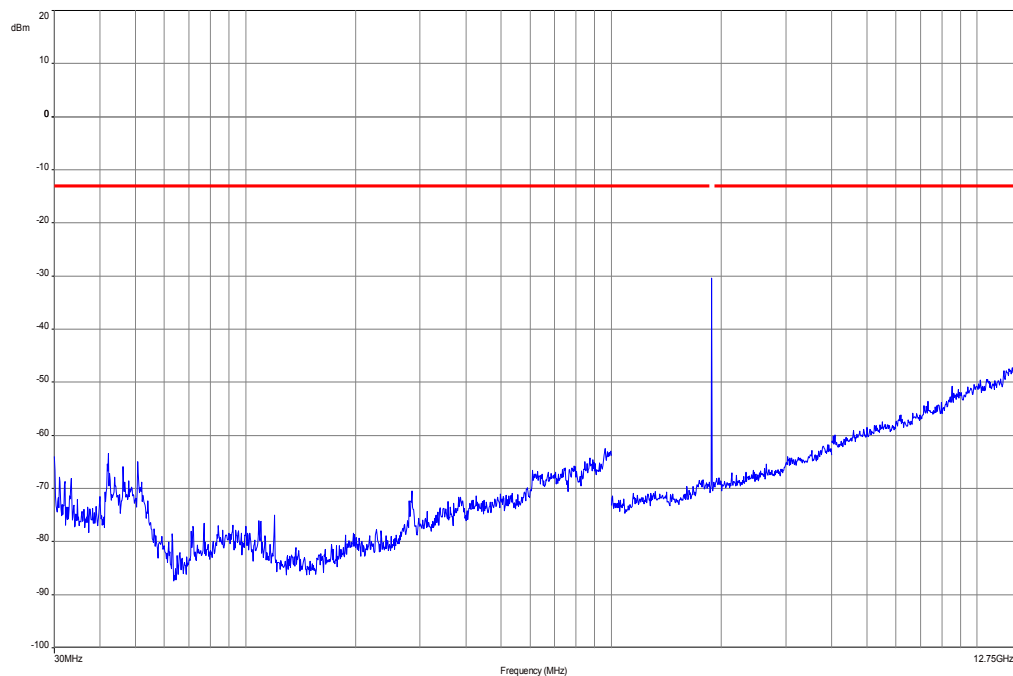
Plot 11: Channel 661 (30 MHz – 12.75 GHz), EDGE
