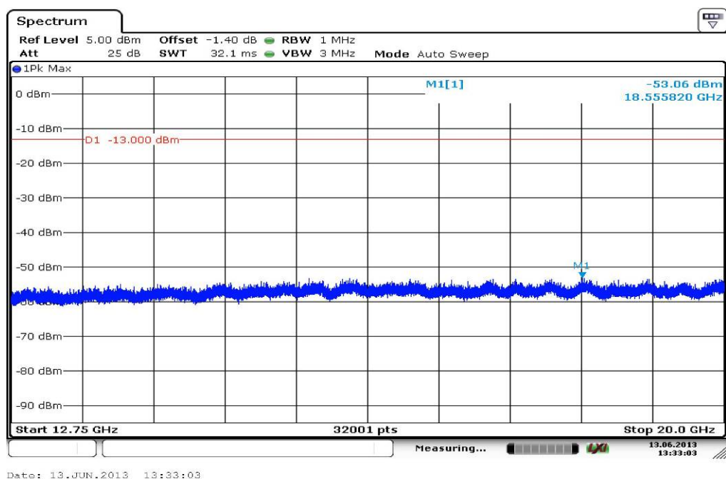
Plot 6: Channel 9538 (12.75 GHz – 20 GHz), voice
