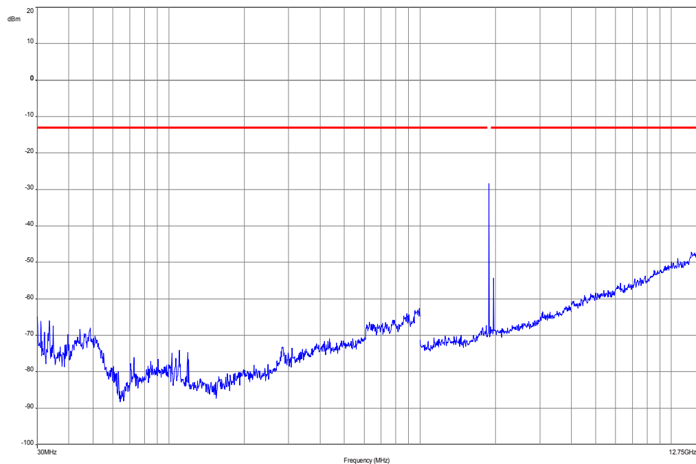
Plot 3: Channel 661 (30 MHz – 12.75 GHz), GSM
