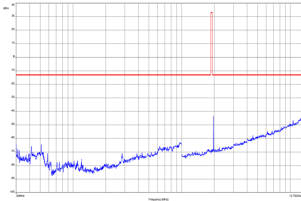
Plot 3: Channel 9400 (30 MHz – 12.75 GHz), HSUPA
