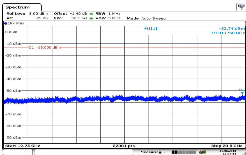
Plot 2: Channel 9262 (12.75 GHz – 20 GHz), HSUPA
