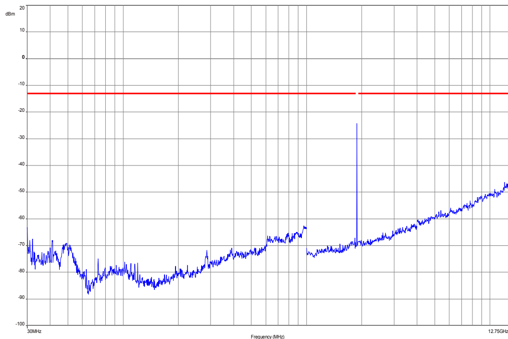
Plot 7: Channel 512 (30 MHz – 12.75 GHz), GPRS
