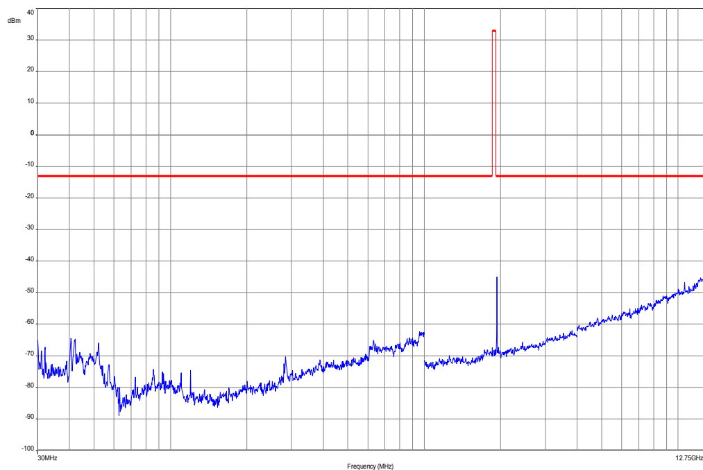
Plot 1: Channel 9262 (30 MHz – 12.75 GHz), HSUPA
