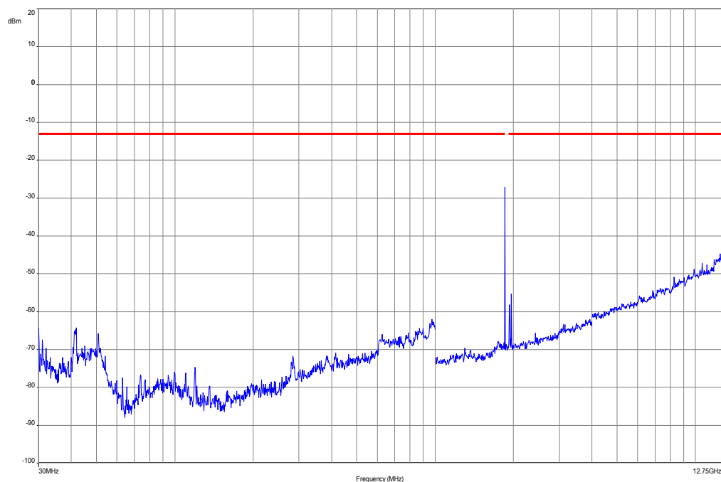
Plot 9: Channel 512 (30 MHz – 12.75 GHz), EDGE
