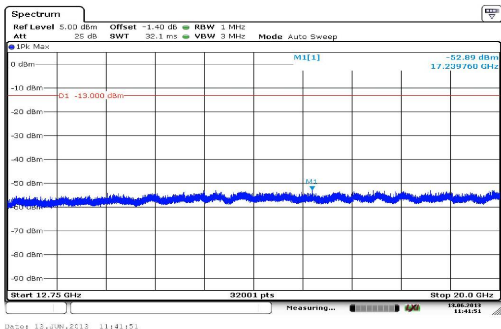
Plot 8: Channel 512 (12 GHz - 20 GHz), GPRS
