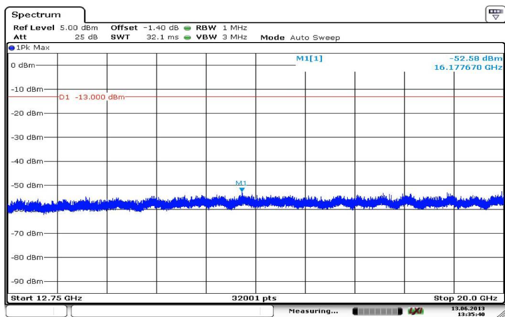
Plot 6: Channel 9538 (12.75 GHz – 20 GHz), HSUPA
