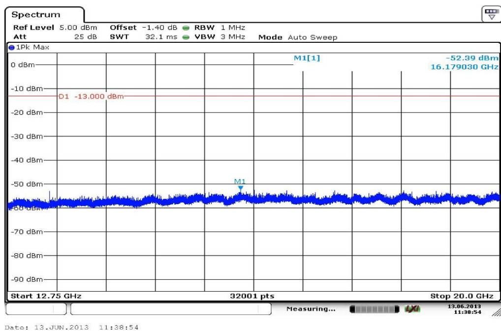
Plot 6: Channel 810 (12 GHz - 20 GHz), GSM
