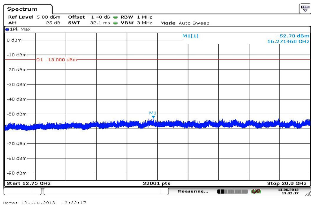
Plot 4: Channel 9400 (12.75 GHz – 20 GHz), voice
