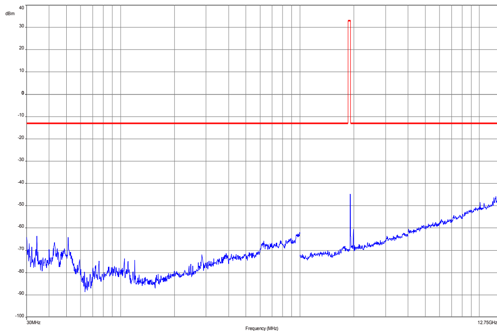
Plot 5: Channel 9538 (30 MHz – 12.75 GHz), HSUPA
