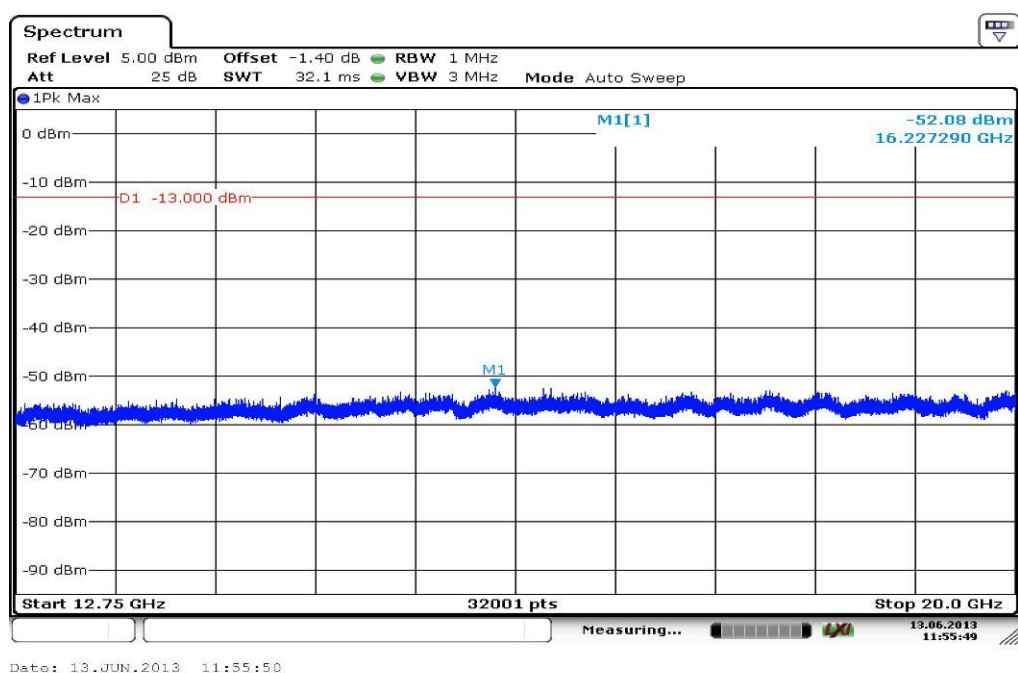
Plot 10: Channel 512 (12 GHz - 20 GHz), EDGE
