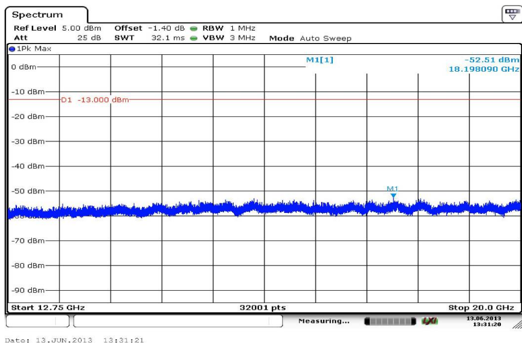
Plot 2: Channel 9262 (12.75 GHz – 20 GHz), voice
