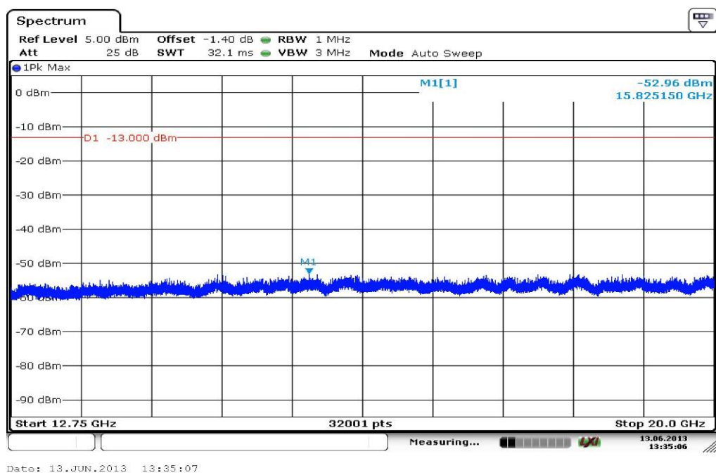
Plot 4: Channel 9400 (12.75 GHz – 20 GHz), HSUPA
