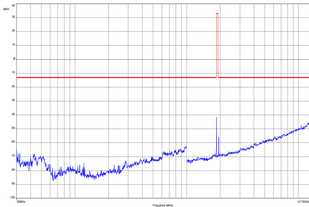
Plot 1: Channel 9262 (30 MHz – 12.75 GHz), voice
