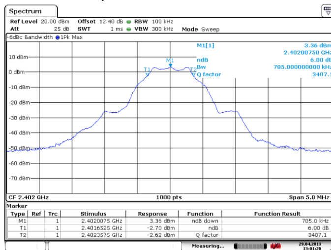
Figure 4-59: 6 dB Bandwidth LE, Channel 0
