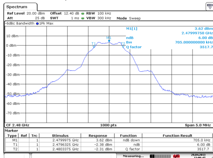
Figure 4-61: 6 dB Bandwidth LE, Channel 39
