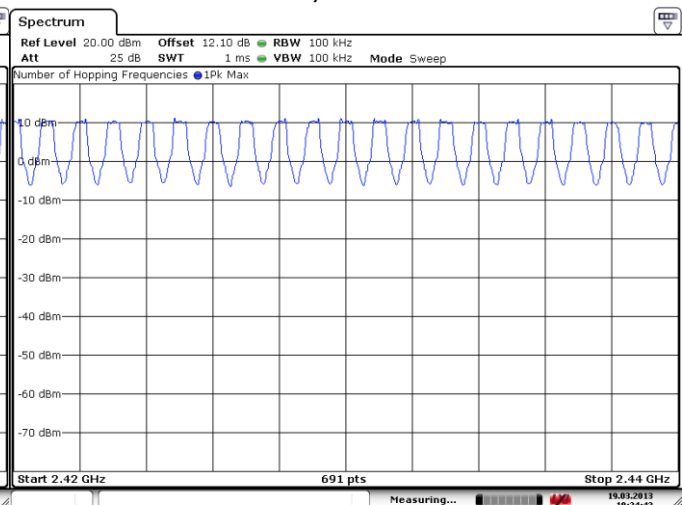
Figure 4-14: Number of Hopping Frequencies Static PBRS, DH5
