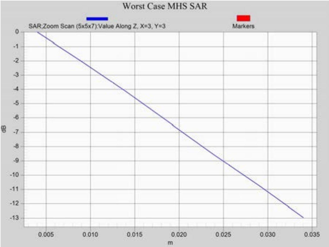
Z axis plot for the worst case hot spot configuration
