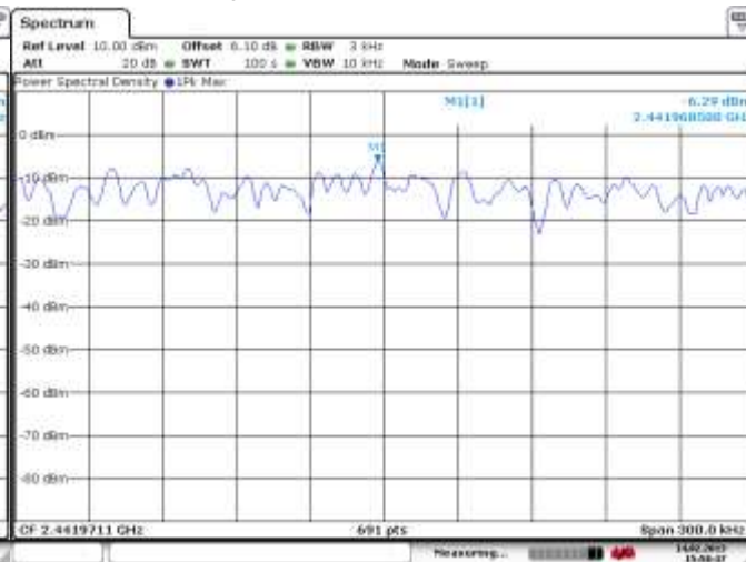
Figure 1-65: Peak Power Spectral Density LE, Channel 20
