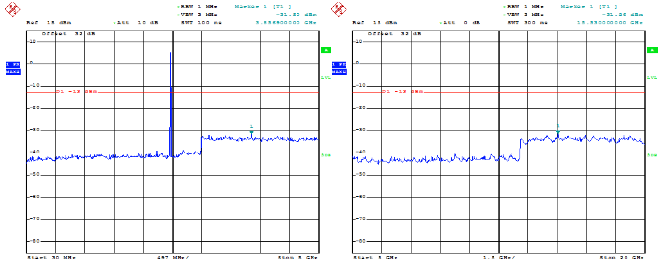
Figure 1-53: Spurious RF Conducted Emissions Single Freq., Static PBRS, 2-DH5
