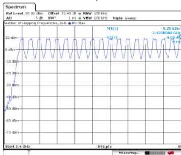
Figure 1-13: Number of Hopping Frequencies Static PBRs, DH5
