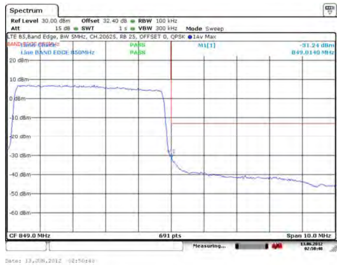
Figure 1-38d: Band 5 High Channel Mask, 5MHz BW, RB=25
