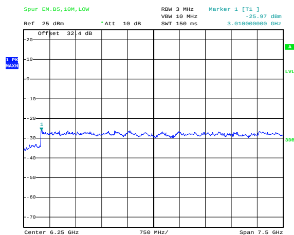
Figure 1-2d: Band 5, Spurious Conducted Emissions, Low channel, 10MHz BW (RB= 50)
