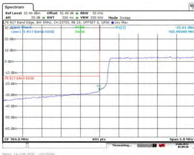
Figure 1-30f: Band 17 Low Channel Mask, 5MHz BW, RB=25
