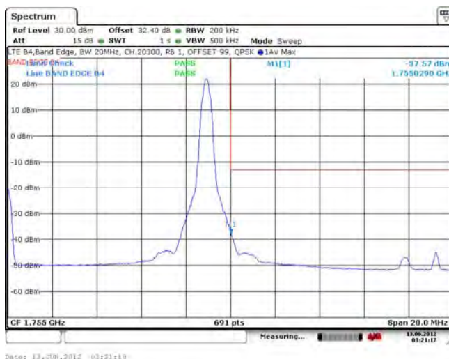
Figure 1-44e: Band 4 High Channel Mask, 20MHz BW, RB=1
