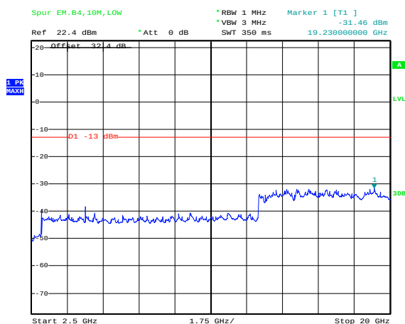
Figure 1-8e: Band 4, Spurious Conducted Emissions, Low channel, 10MHz BW (RB= 50)
