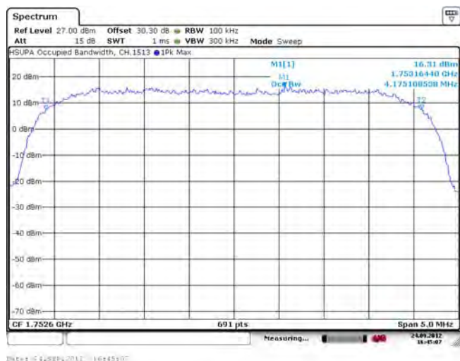
Figure 1-73b: Occupied Bandwidth, Band 4 High Channel
