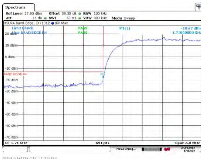
Figure 1-74b: Band 4 , Low Channel Mask
