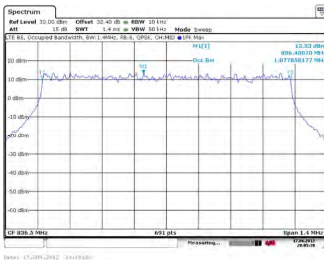
Figure 1-26d: Occupied Bandwidth, Band 5 Middle Channel, 1.4MHz BW, RB=6
