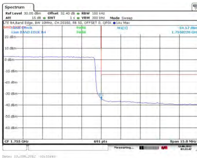
Figure 1-40e: Band 4 High Channel Mask, 10MHz BW, RB=50
