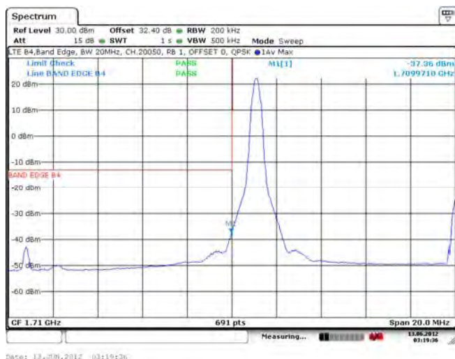
Figure 1-43e: Band 4 Low Channel Mask, 20MHz BW, RB=1
