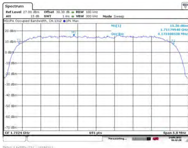
Figure 1-71b: Occupied Bandwidth, Band 4 Low Channel
