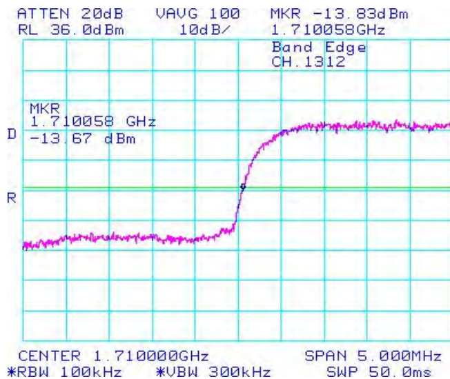
Figure 1-63b: Channel Mask, Low Channel Band 4
