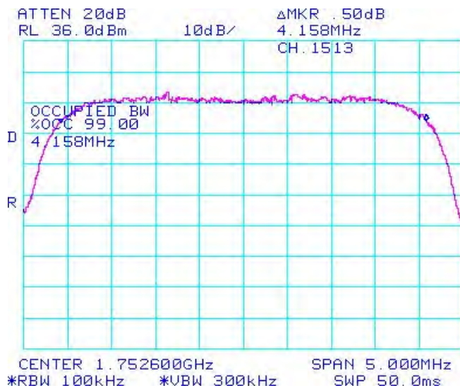
Figure 1-59b: Occupied Bandwidth, Band 4 High Channel
