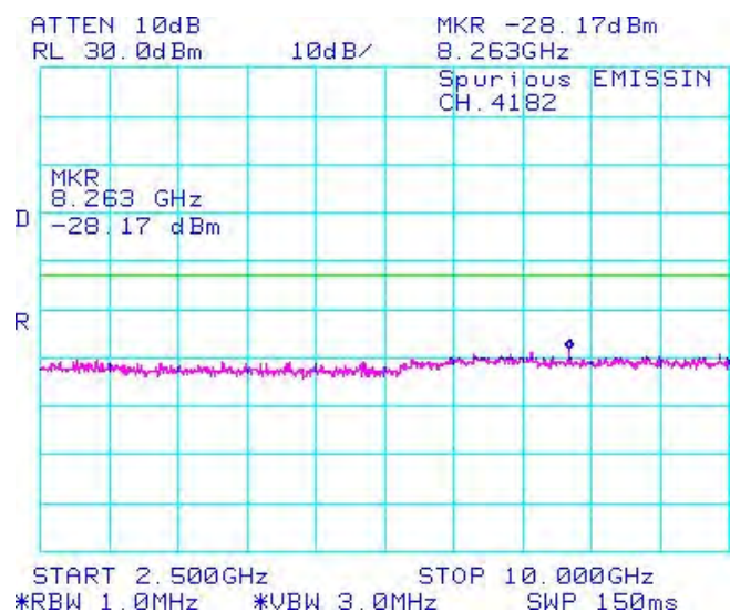
Figure 1-4b: Band 5, Spurious Conducted Emissions, Middle channel
