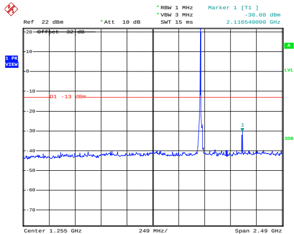
Figure 1-65b: Band 4 , Spurious Conducted Emissions, Low channel
