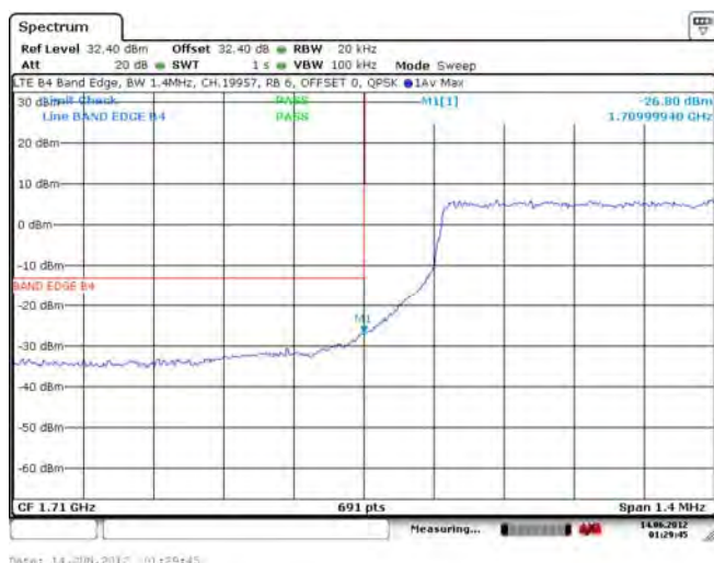
Figure 1-41e: Band 4 Low Channel Mask, 1.4MHz BW, RB=6
