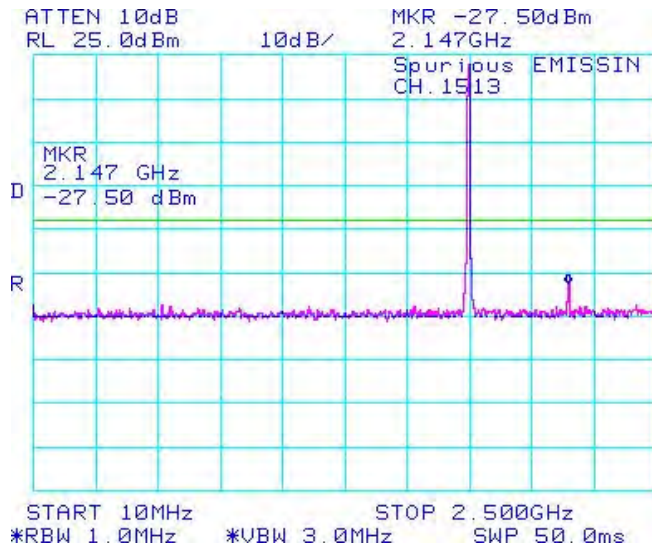
Figure 1-55b: Band 4, Spurious Conducted Emissions, High channel
