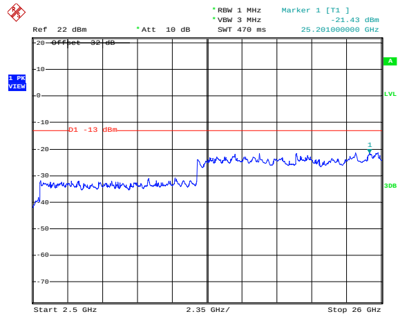
Figure 1-66b: Band 4 , Spurious Conducted Emissions, Low channel
