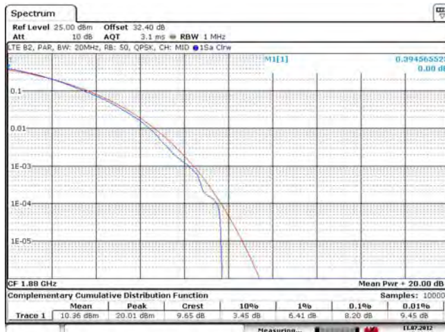
Figure 1-34c: Band 2 Middle Channel PAR, 20 MHz BW, RB = 50
