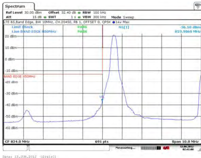
Figure 1-41d: Band 5 Low Channel Mask, 10MHz BW, RB=1
