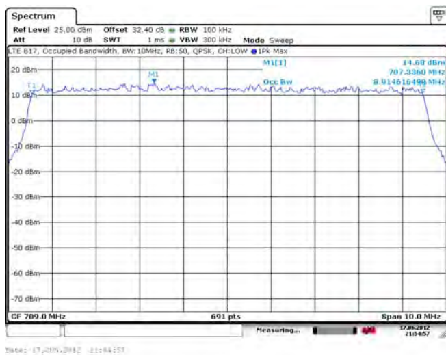
Figure 1-13f: Occupied Bandwidth, Band 17 Low Channel, 10MHz BW, RB=50
