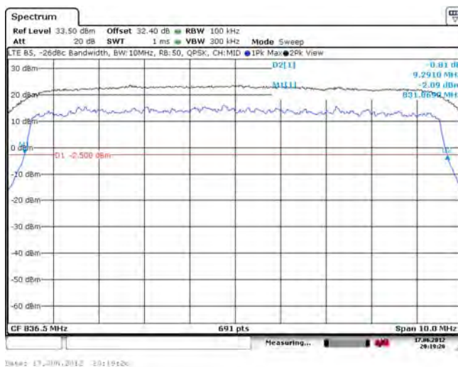
Figure 1-29d: -26 dBc Bandwidth, Band 5 Middle Channel, 10MHz BW, RB=50
