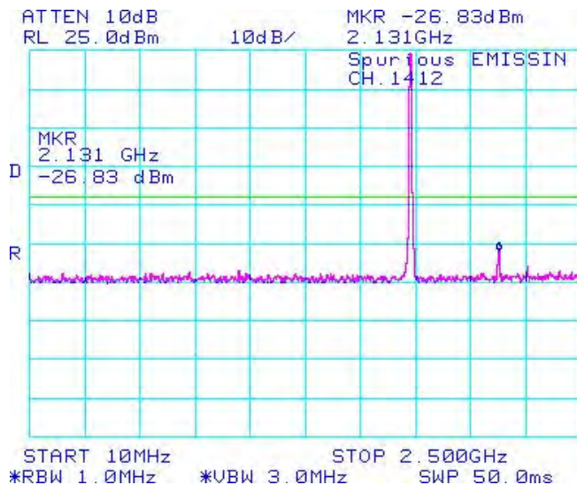
Figure 1-53b: Band 4, Spurious Conducted Emissions, Middle channel
