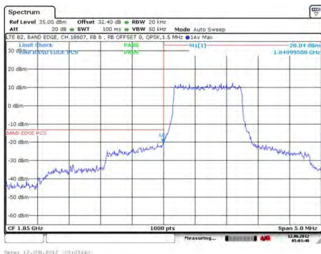
Figure 1-29c: Band 2 Low Channel Mask, 1.4MHz BW, RB = 6
