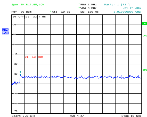
Figure 1-8f: Band 17, Spurious Conducted Emissions, Low channel, 5MHz BW (RB= 25)
