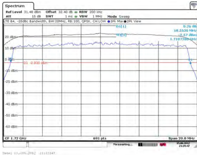
Figure 1-28e: -26 dBc Bandwidth, Band 4 Low Channel, 20MHz BW, RB=100
