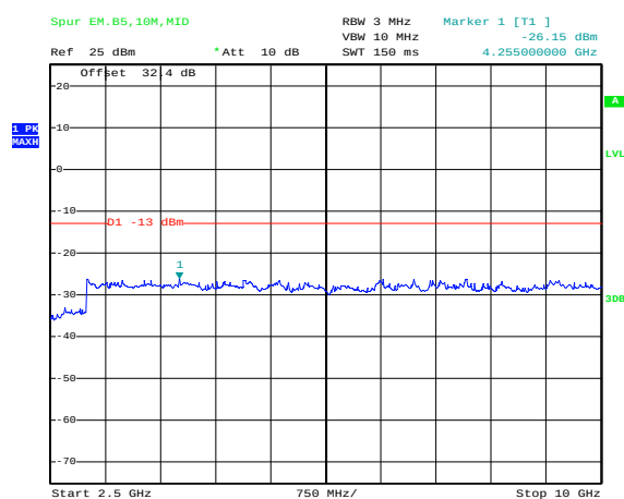
Figure 1-4d: Band 5, Spurious Conducted Emissions, Middle channel, 10MHz BW (RB= 50)
