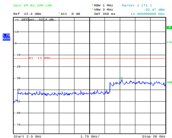
Figure 1-8c: Band 2, Spurious Conducted Emissions, Low channel, 10MHz BW (RB= 50)
