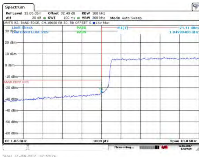
Figure 1-27c: Band 2 Low Channel Mask, 10MHz BW, RB = 50
