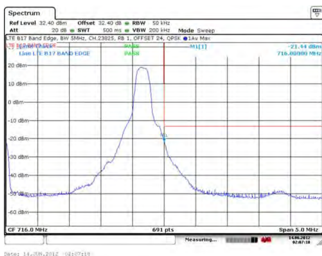
Figure 1-31f: Band 17 High Channel Mask, 5MHz BW, RB=1
