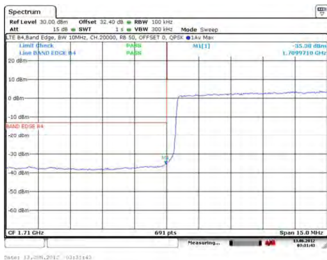
Figure 1-39: Band 4 Low Channel Mask, 10MHz BW, RB=50
