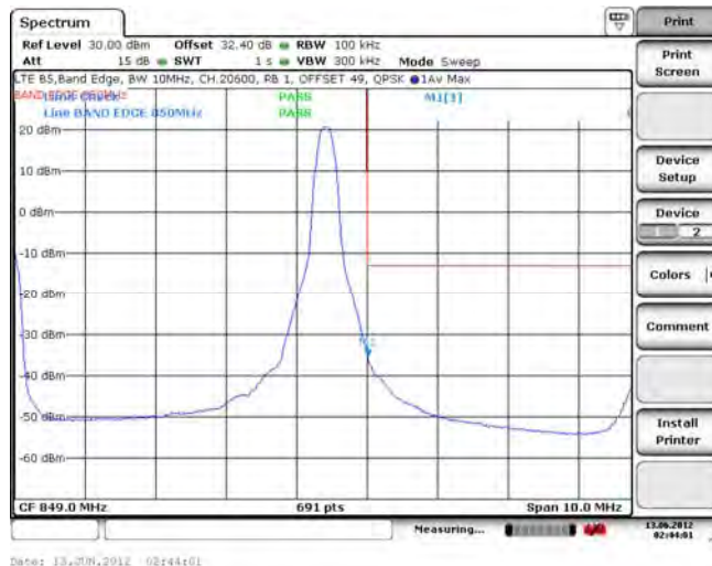
Figure 1-42d: Band 5 High Channel Mask, 10MHz BW, RB=1
