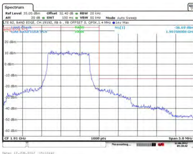
Figure 1-30c: Band 2 High Channel Mask, 1.4MHz BW, RB = 6
