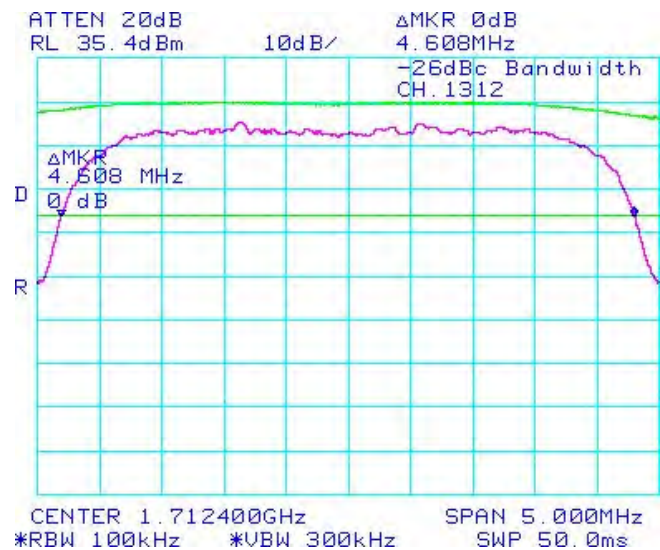
Figure 1-60b: -26 dBc Bandwidth, Band 4 Low Channel
