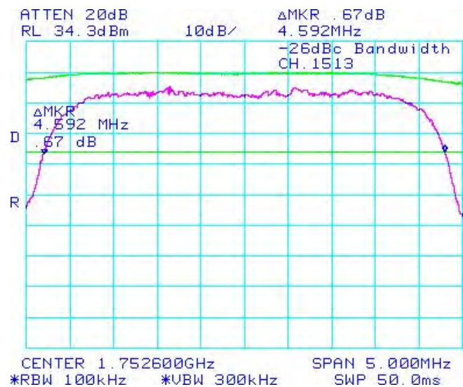
Figure 1-62b: -26 dBc Bandwidth, Band 4 High Channel
