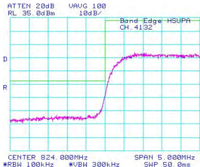
Figure 1-47b: Band 5 , Low Channel Mask
