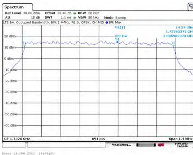
Figure 1-26e: Occupied Bandwidth, Band 4 Middle Channel, 1.4MHz BW, RB=6
