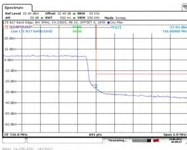
Figure 1-32f: Band 17 High Channel Mask, 5MHz BW, RB=25
