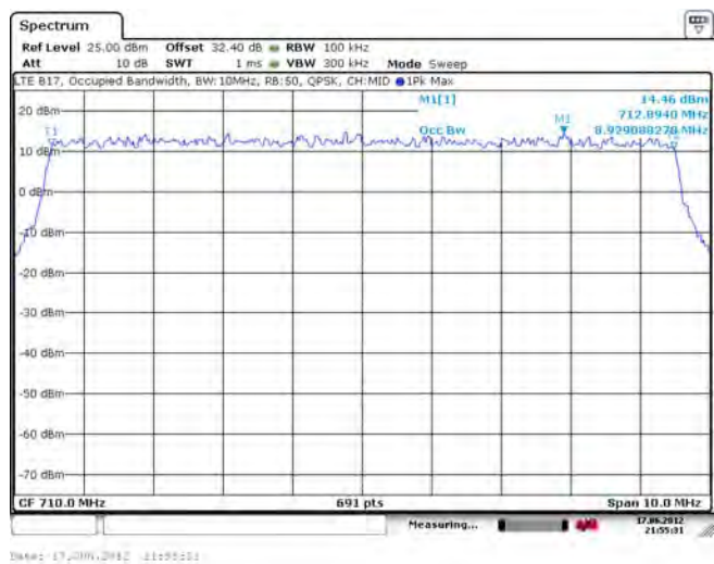
Figure 1-14f: Occupied Bandwidth, Band 17 Middle Channel, 10MHz BW, RB=50
