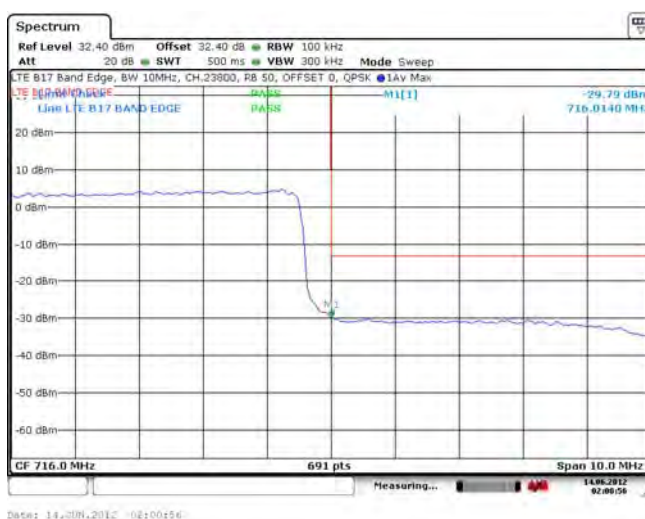
Figure 1-28f: Band 17 High Channel Mask, 10MHz BW, RB=50
