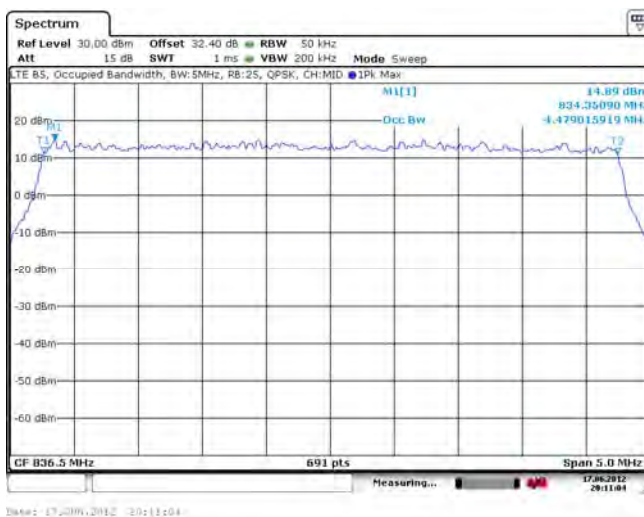
Figure 1-23d: Occupied Bandwidth, Band 5 Middle Channel, 5MHz BW, RB=25
