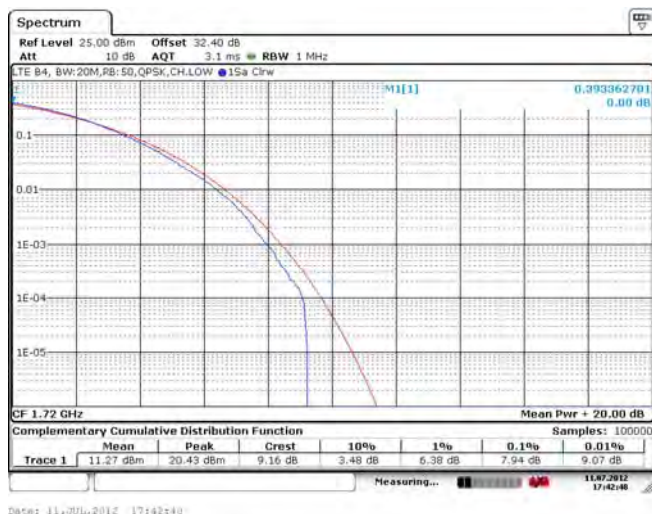
Figure 1-45e: Band 4 Low Channel PAR, 20MHz BW, RB=50
