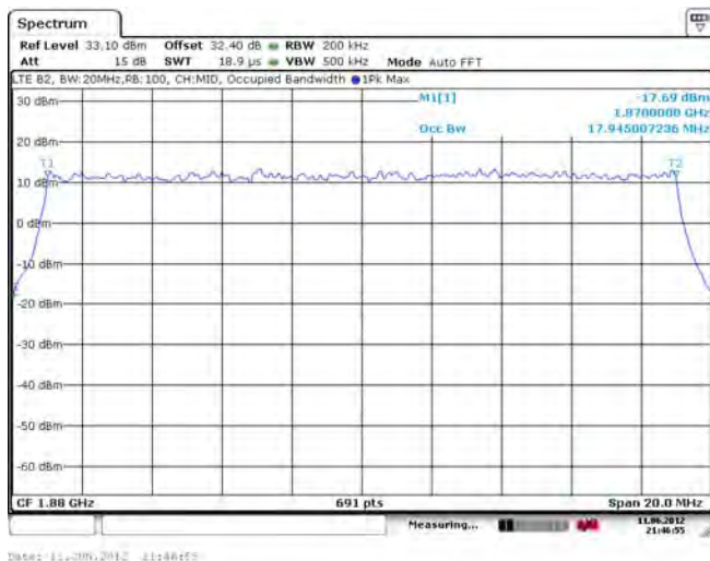
Figure 1-20c: Occupied Bandwidth, Band 2 Middle Channel, 20MHz BW (RB= 100)
