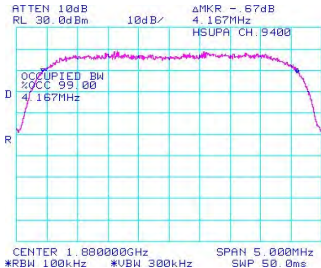
Figure 1-45b: Occupied Bandwidth, Band 2 Middle Channel
