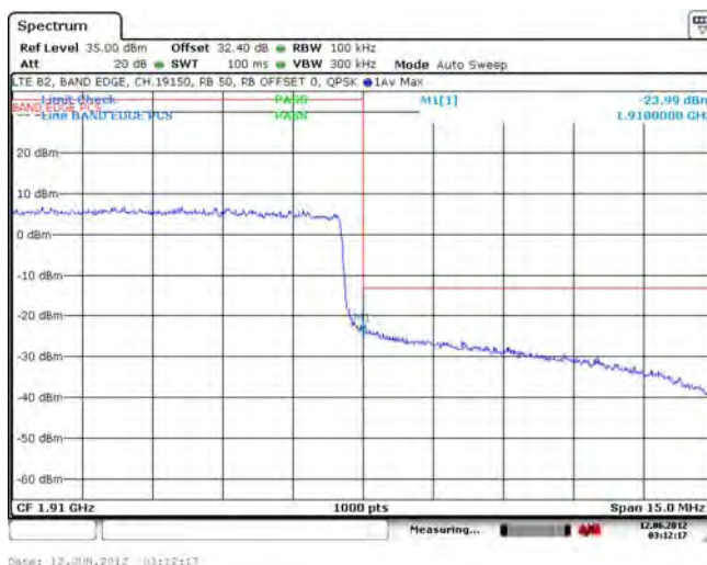
Figure 1-28c: Band 2 High Channel Mask, 10MHz BW, RB = 50
