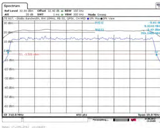
Figure 1-20f: -26 dBc Bandwidth, Band 17 Middle Channel, 10MHz BW, RB=50
