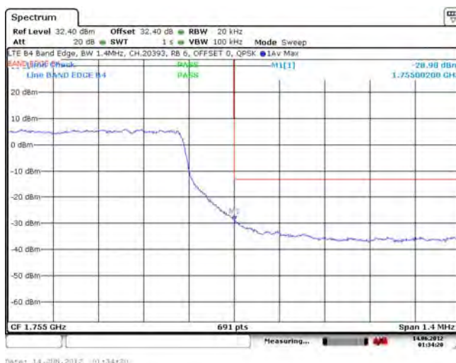
Figure 1-42e: Band 4 High Channel Mask, 1.4MHz BW, RB=6
