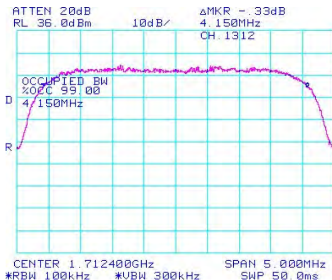
Figure 1-57b: Occupied Bandwidth, Band 4 Low Channel
