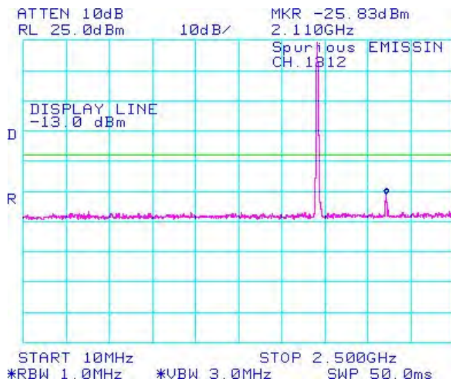
Figure 1-51b: Band 4, Spurious Conducted Emissions, Low channel
