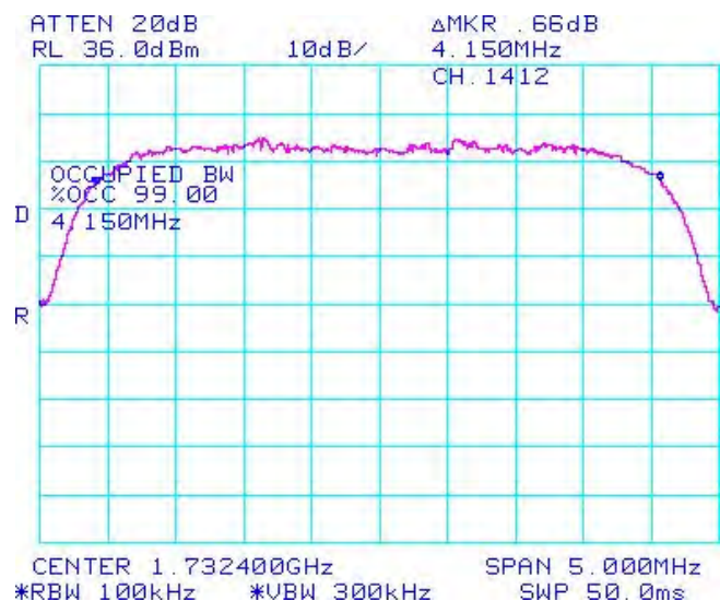
Figure 1-58b: Occupied Bandwidth, Band 4 Middle Channel
