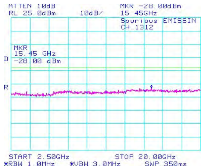
Figure 1-52b: Band 4, Spurious Conducted Emissions, Low channel
