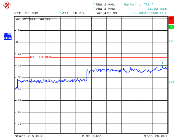
Figure 1-70b: Band 4 , Spurious Conducted Emissions, High Channel
