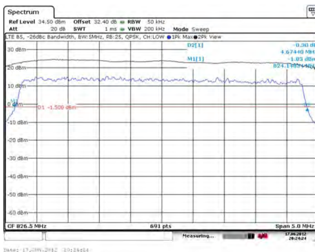
Figure 1-31d: -26 dBc Bandwidth, Band 5 Low Channel, 5MHz BW, RB=25
