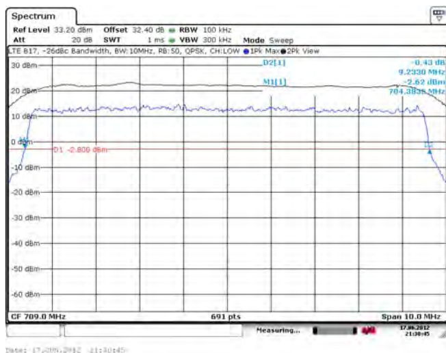
Figure 1-19f: -26 dBc Bandwidth, Band 17 Low Channel, 10MHz BW, RB=50
