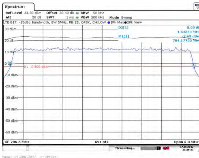
Figure 1-22f: -26 dBc Bandwidth, Band 17 Low Channel, 5MHz BW, RB=25
