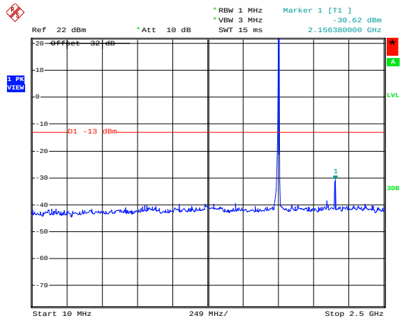
Figure 1-69b: Band 4 , Spurious Conducted Emissions, High Channel
