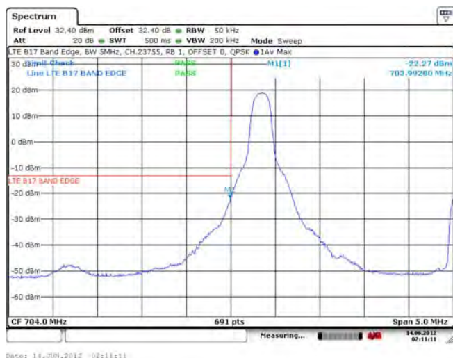
Figure 1-29f: Band 17 Low Channel Mask, 5MHz BW, RB=1
