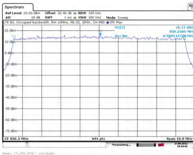
Figure 1-20d: Occupied Bandwidth, Band 5 Middle Channel, 10MHz BW, RB=50
