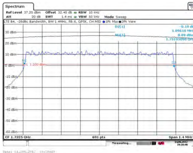
Figure 1-35e: -26 dBc Bandwidth, Band 4 Middle Channel, 1.4MHz BW, RB=6
