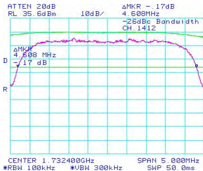
Figure 1-61b: -26 dBc Bandwidth, Band 4 Middle Channel
