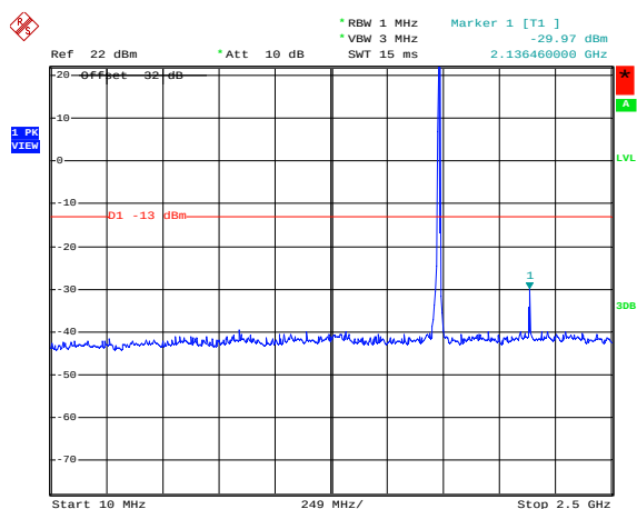
Figure 1-67b: Band 4 , Spurious Conducted Emissions, Middle channel
