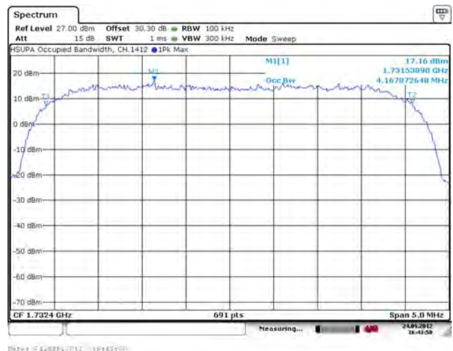
Figure 1-72b: Occupied Bandwidth, Band 4 Middle Channel
