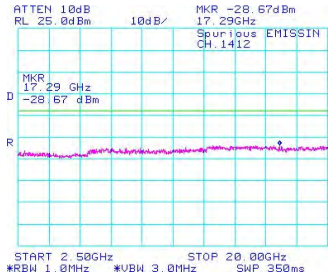
Figure 1-54b: Band 4, Spurious Conducted Emissions, Middle channel
