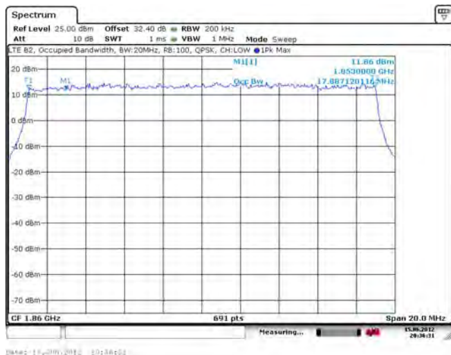
Figure 1-19c: Occupied Bandwidth, Band 2 Low Channel, 20MHz BW (RB= 100)
