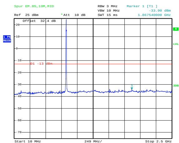
Figure 1-3d: Band 5, Spurious Conducted Emissions, Middle channel, 10MHz BW (RB= 50)
