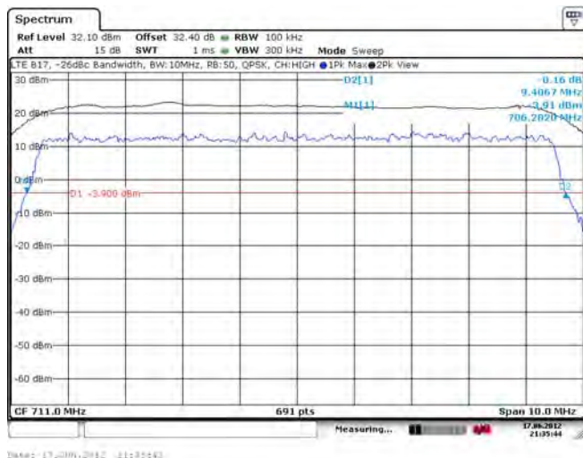
Figure 1-21f: -26 dBc Bandwidth, Band 17 High Channel, 10MHz BW, RB=50
