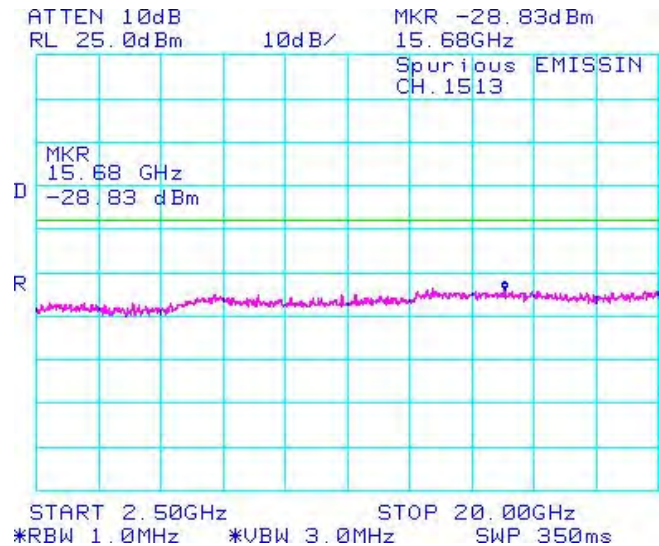
Figure 1-56b: Band 4, Spurious Conducted Emissions, High channel
