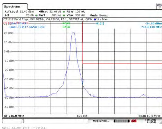
Figure 1-27f: Band 17 High Channel Mask, 10MHz BW, RB=1
