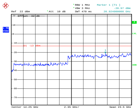
Figure 1-68b: Band 4 , Spurious Conducted Emissions, Middle channel
