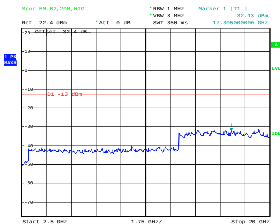
Figure 1-6c: Band 2, Spurious Conducted Emissions, High Channel, 20MHz BW (RB= 100)
