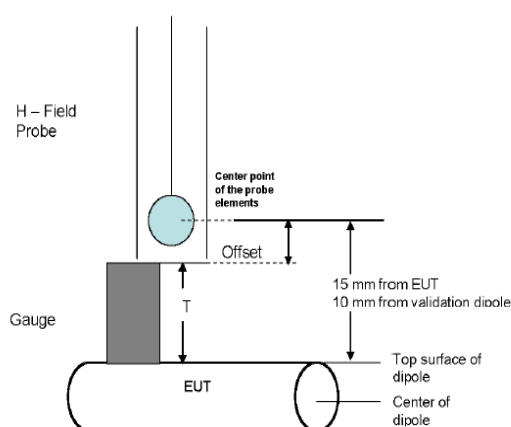
H-Field Probe (H3DV6)
