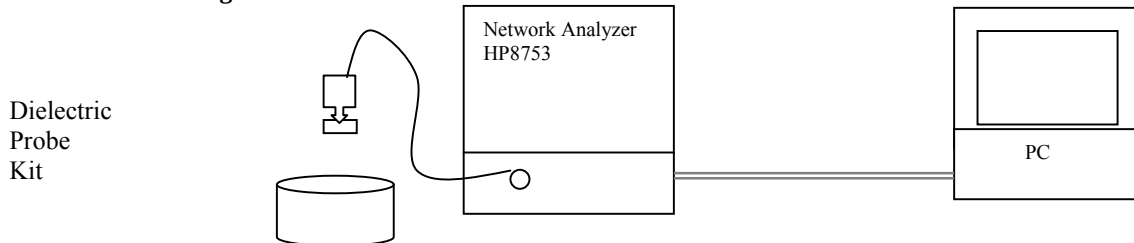
Figure 6.2.1. Test configuration
