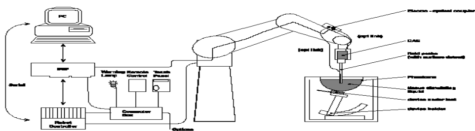
Figure 2.1.1. System Description
