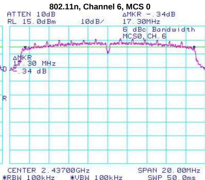
Figure 4-8: 6 dB Bandwidth
