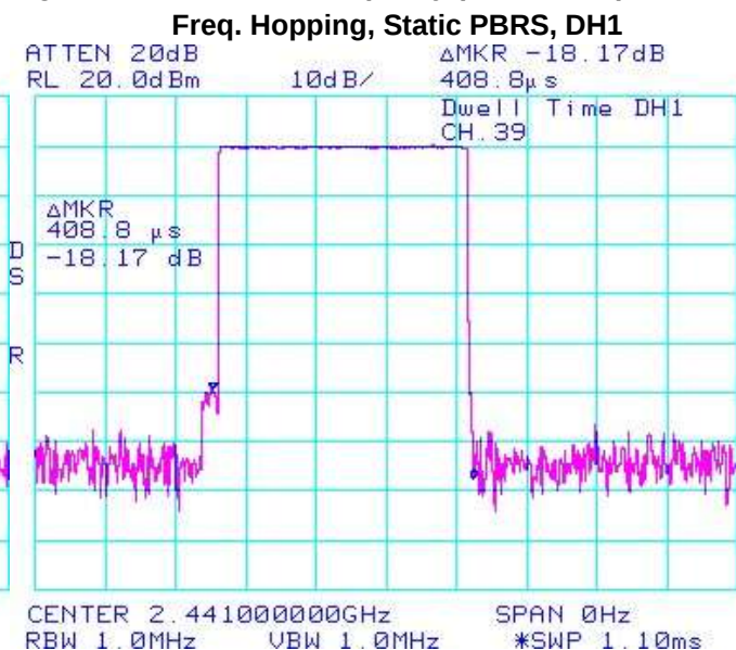
Figure 3-18: Time of Occupancy (Dwell Time)
