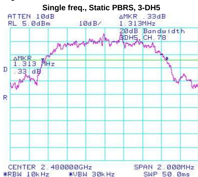
Figure 3-9: 20 dB Bandwidth
