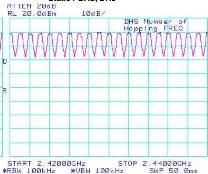
Figure 3-14: Number of Hopping Frequencies
