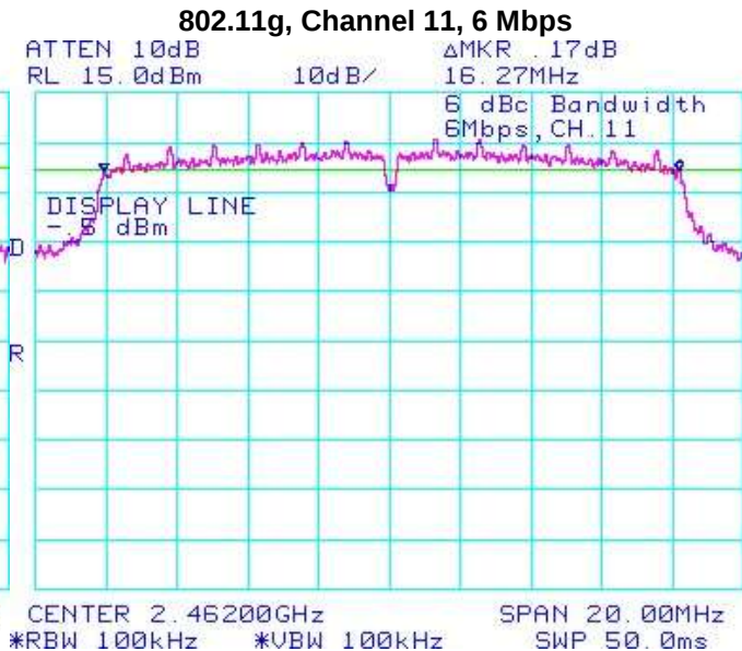
Figure 4-6: 6 dB Bandwidth
