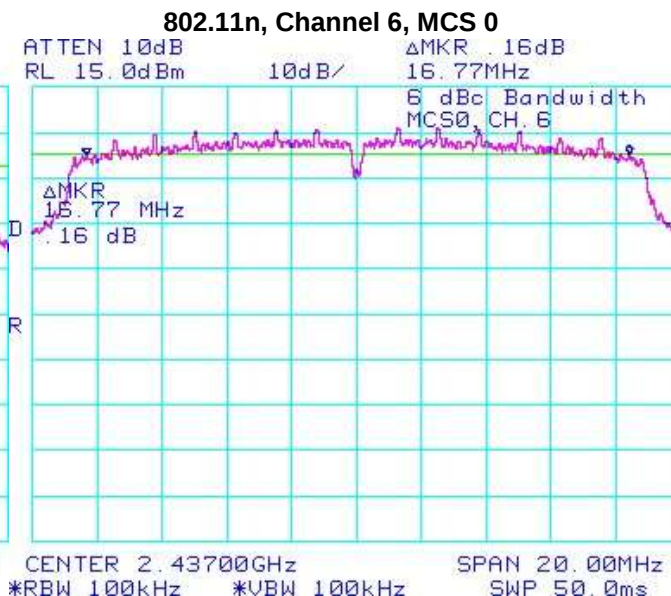
Figure 4-8: 6 dB Bandwidth
