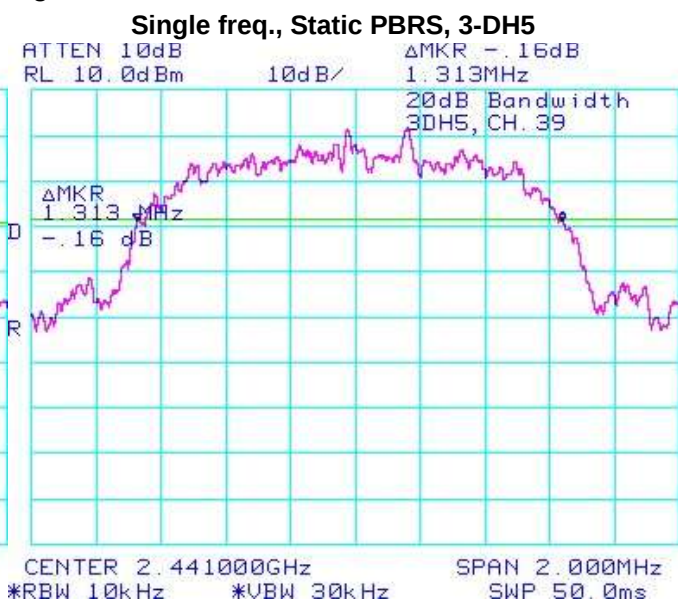
Figure 3-8: 20 dB Bandwidth
