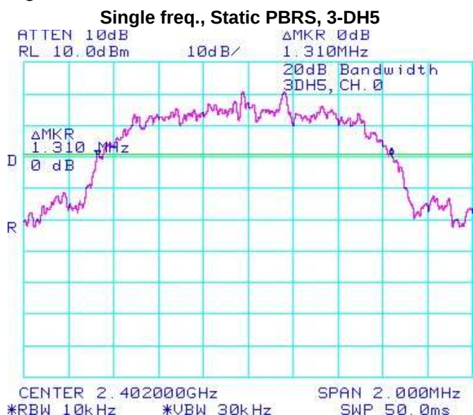
Figure 3-7: 20 dB Bandwidth
