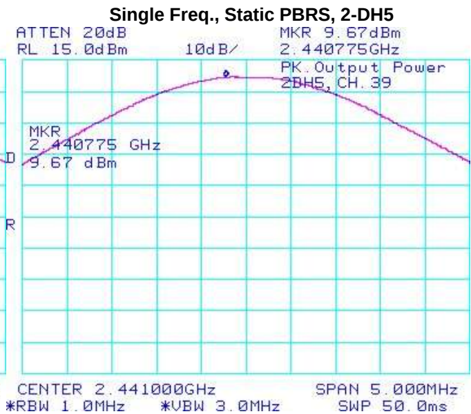
Figure 3-30: Max. Peak Conducted Output Power
