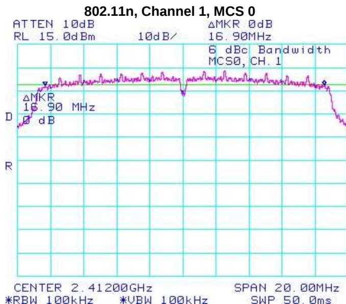
Figure 4-7: 6 dB Bandwidth
