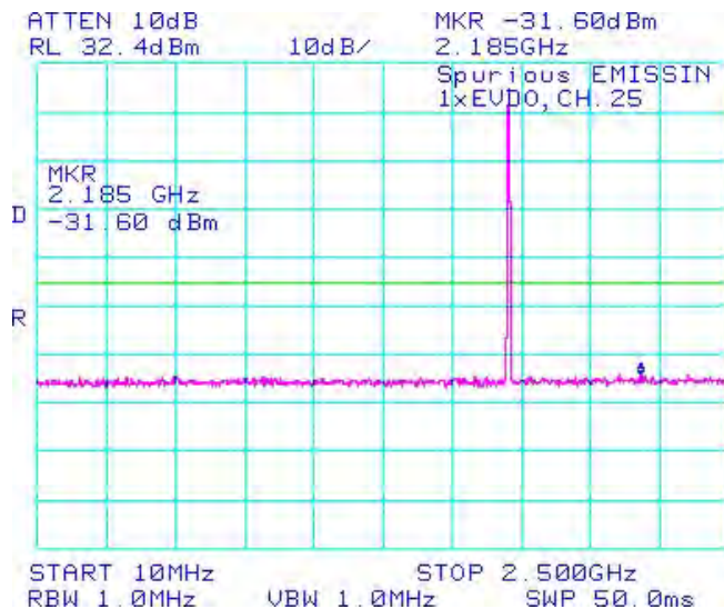
Figure 1-12b: Cellular, Spurious Conducted Emissions, Low channel
