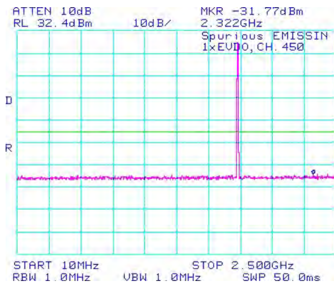
Figure 1-14b: Cellular, Spurious Conducted Emissions, Middle channel
