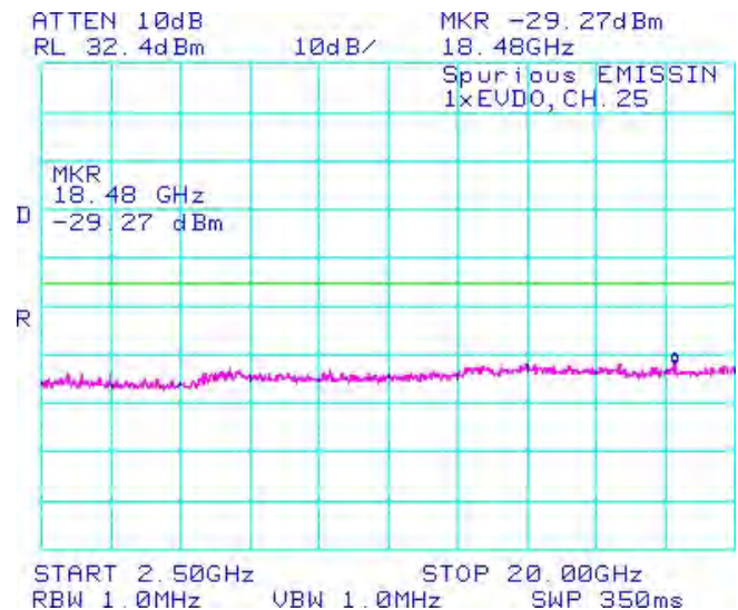
Figure 1-13b: Cellular, Spurious Conducted Emissions, Low channel
