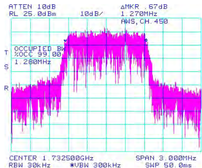
Figure 1-8b: Occupied Bandwidth, Cellular Middle Channel
