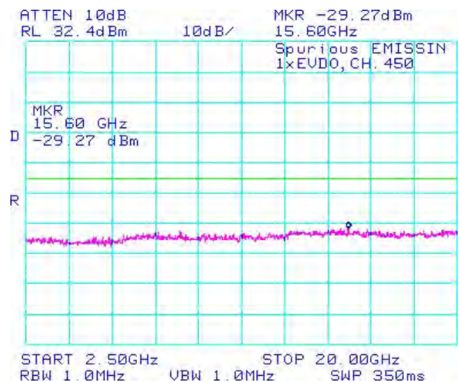
Figure 1-15b: Cellular, Spurious Conducted Emissions, Middle channel
