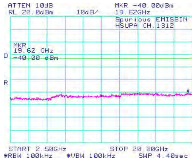
Figure 1-16c: Band 4 , Spurious Conducted Emissions, Low channel
