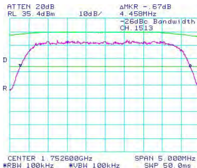
Figure 1-12c: -26 dBc Bandwidth, Band 4 High Channel
