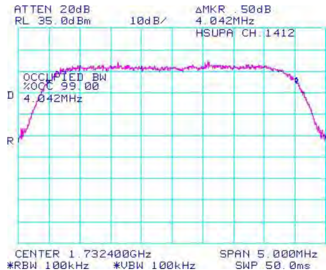
Figure 1-22c: Occupied Bandwidth, Band 4 Middle Channel
