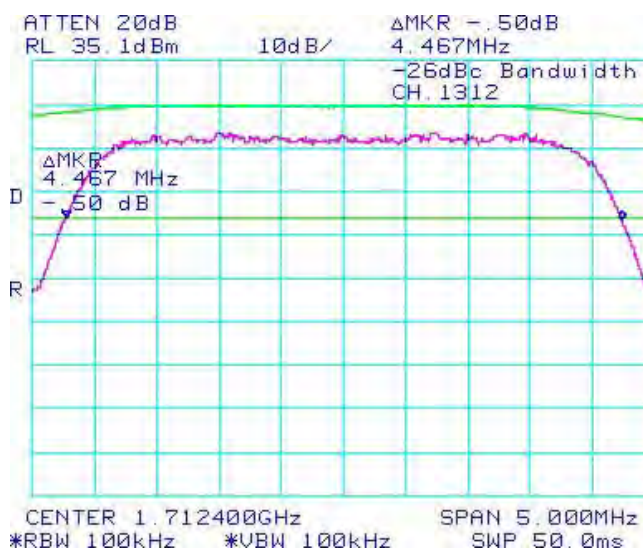
Figure 1-10c: -26 dBc Bandwidth, Band 4 Low Channel
