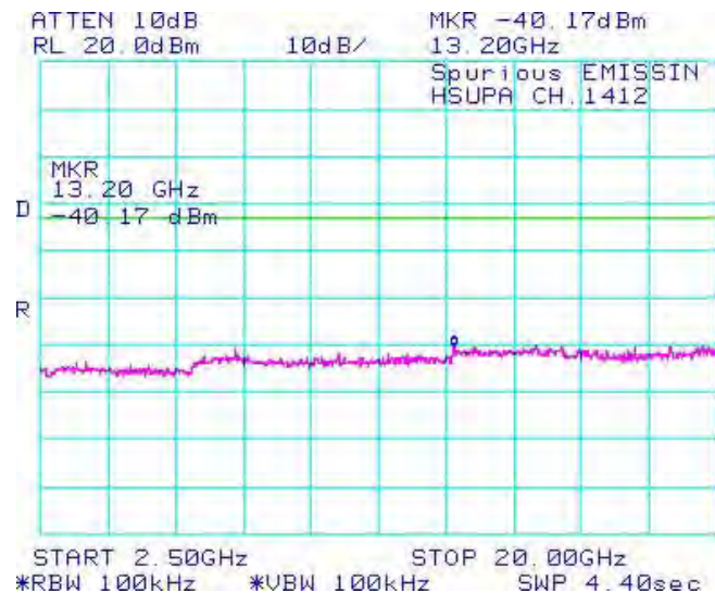
Figure 1-18c: Band 4 , Spurious Conducted Emissions, Middle channel
