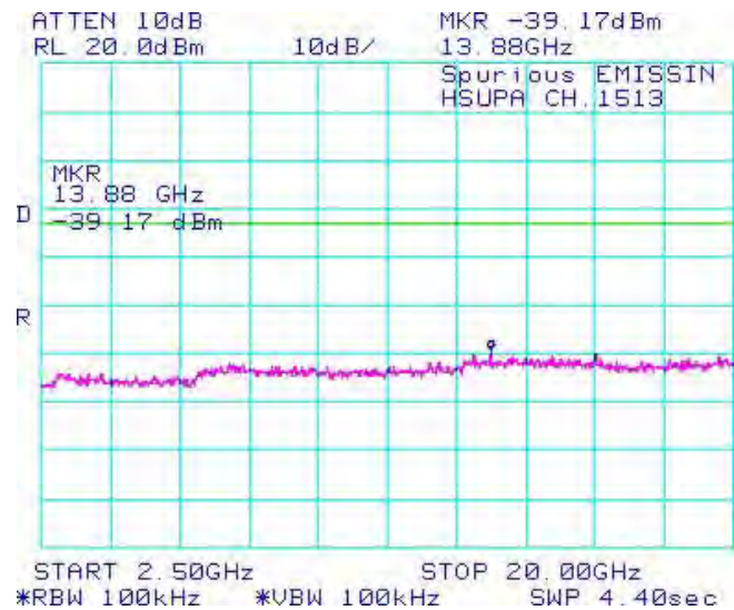
Figure 1-20c: Band 4 , Spurious Conducted Emissions, High Channel
