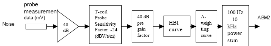
Figure 6.2. ABM2 block diagram
