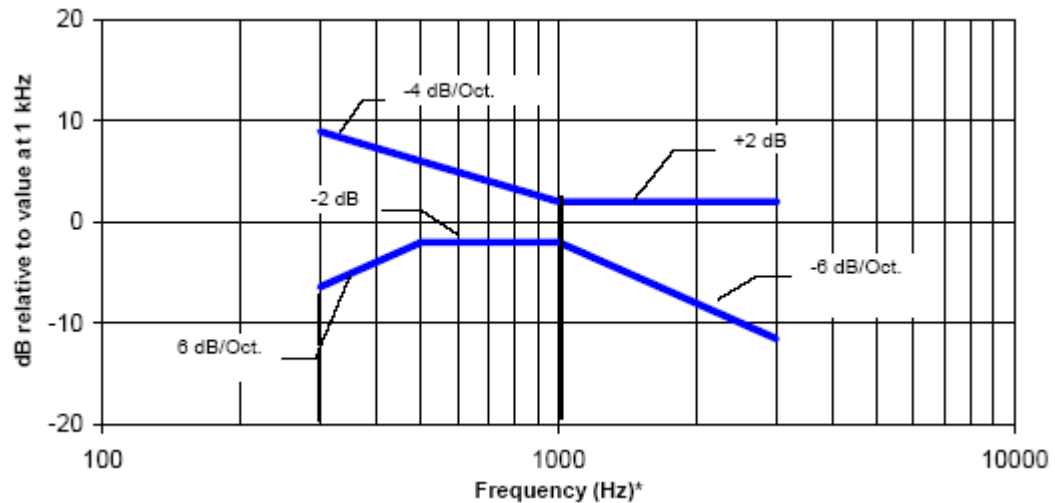
Figure 6.7. Magnetic field frequency response for WDs with a field between 10 dB and -13 dB (A/m) at 1 kHz
