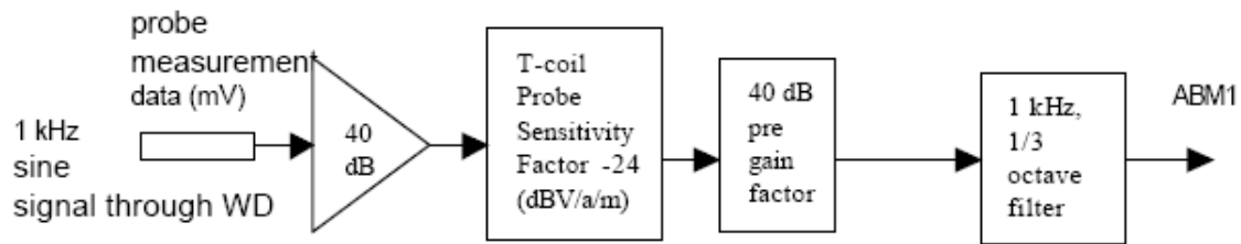
Figure 6.1. ABM1 block diagram
