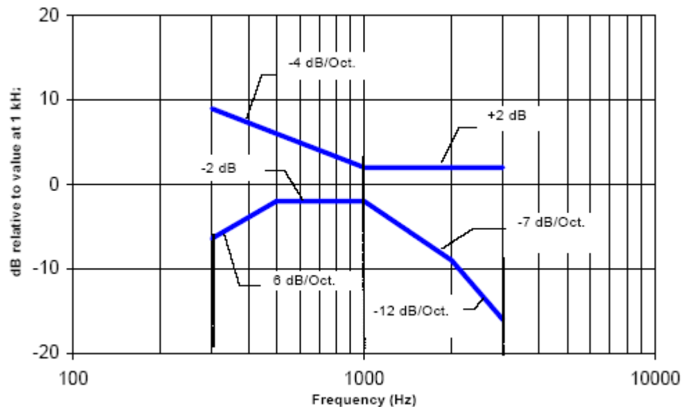
Figure 6.8. Magnetic field frequency response for WDs with a field that exceeds -10 dB(A/m) at 1 kHz
