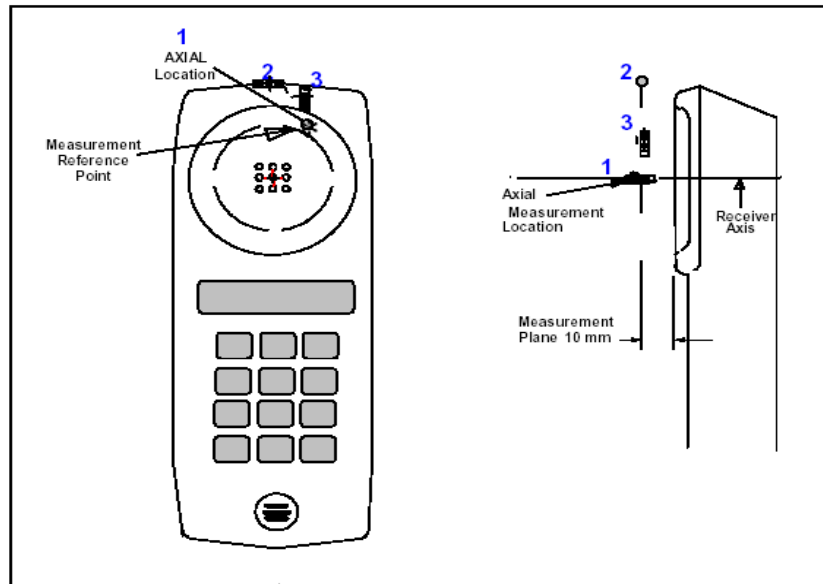
Figure 6.3. Axis & planes for WD audio band magnetic field measurements
