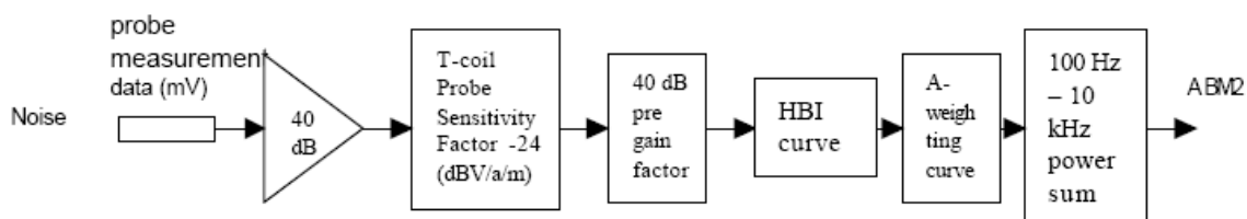
Figure 6.3. ABM2 block diagram
