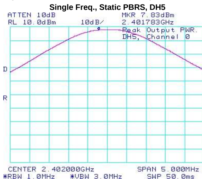
Figure 2-22: Max. Peak Conducted Output Power
