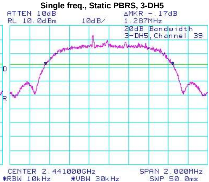
Figure 2-5: 20 dB Bandwidth
