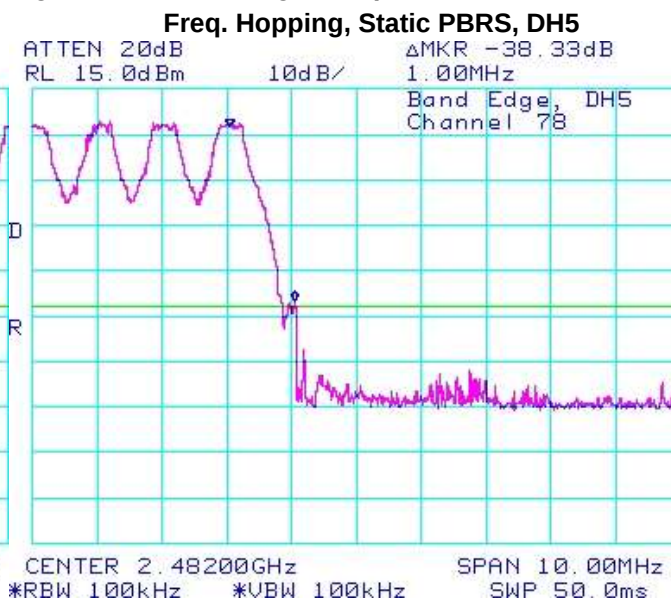
Figure 2-31: Band Edge Compliance
