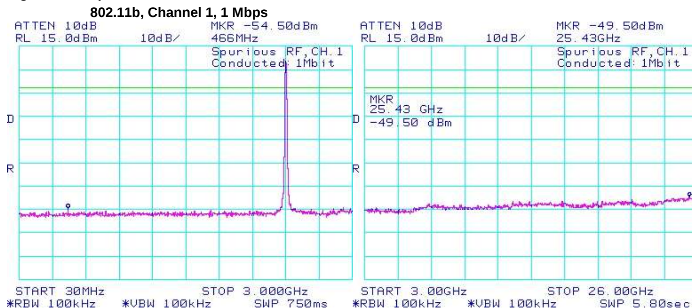
Figure 3-25: Spurious Conducted RF Emissions
