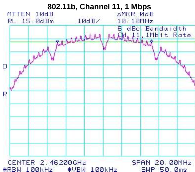
Figure 3-3: 6 dB Bandwidth
