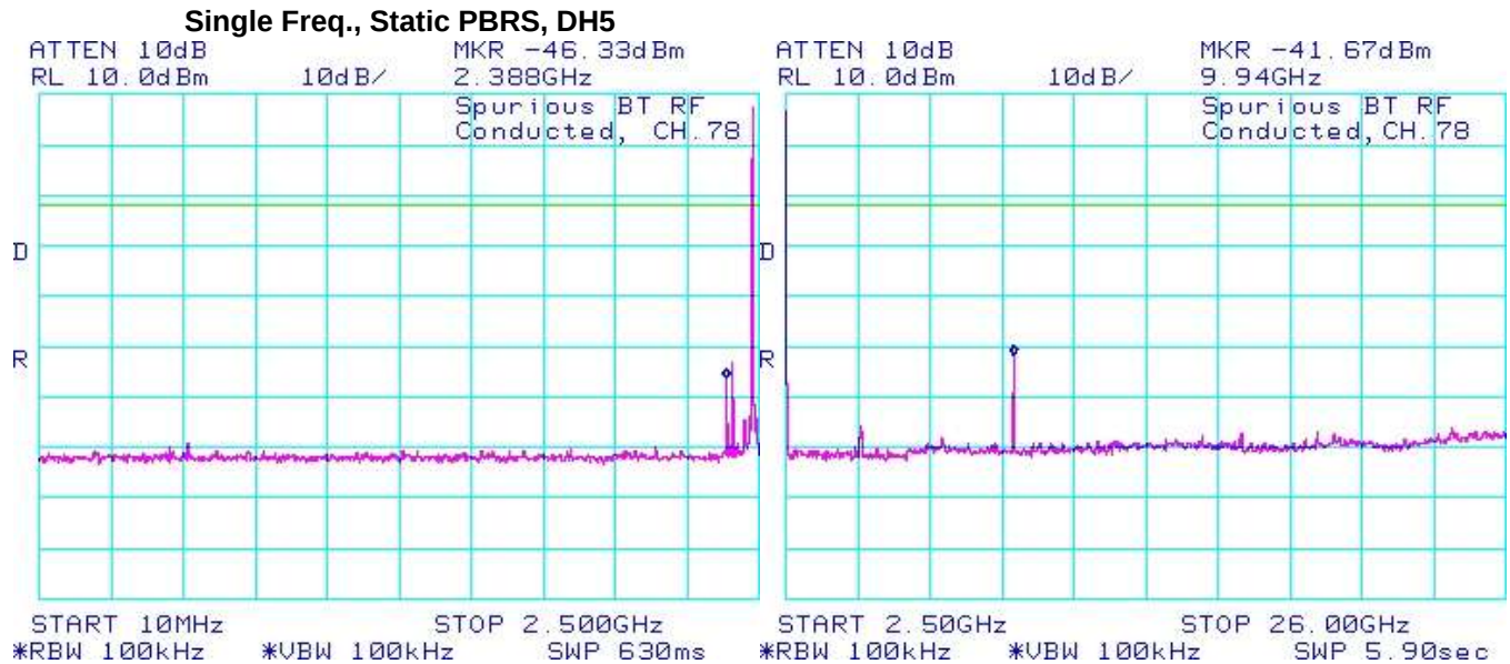
Figure 2-38: Spurious RF Conducted Emissions
