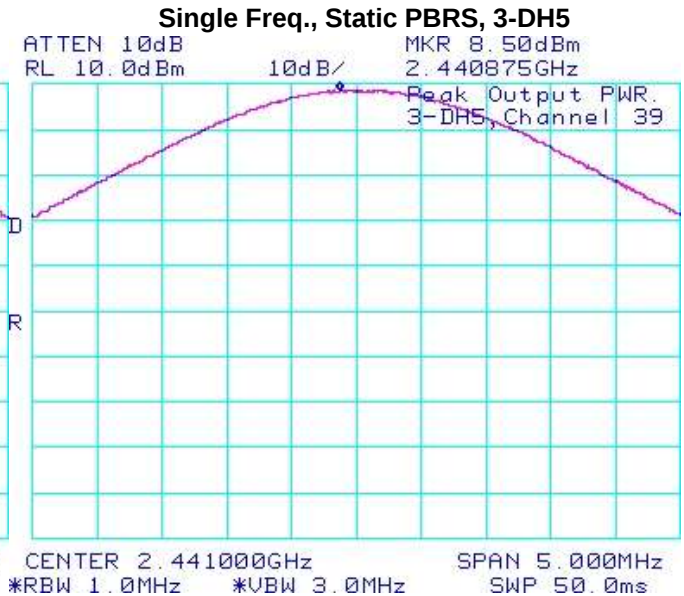
Figure 2-26: Max. Peak Conducted Output Power
