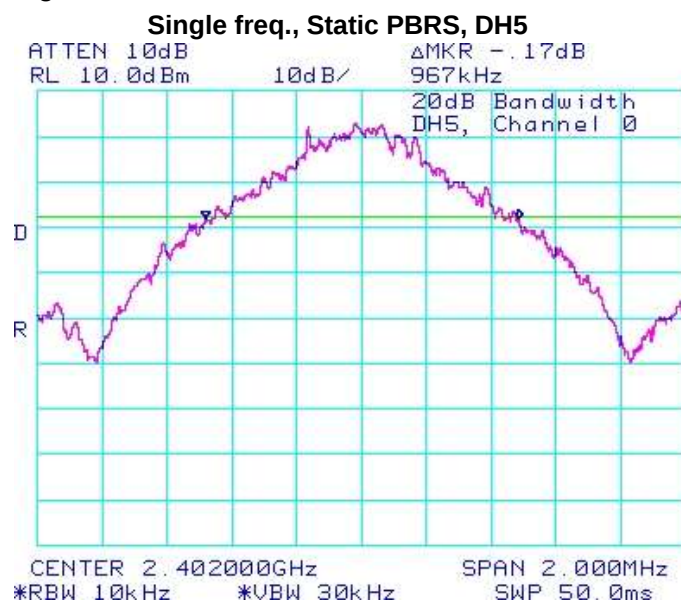
Figure 2-1: 20 dB Bandwidth
