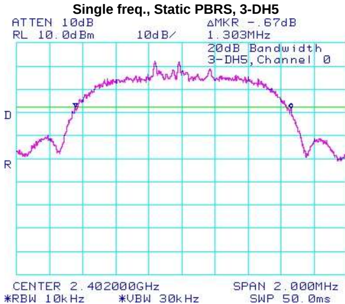
Figure 2-4: 20 dB Bandwidth
