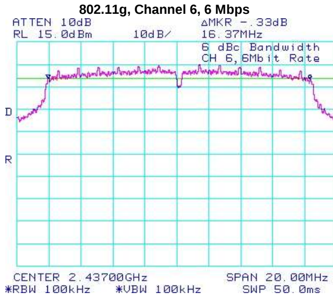
Figure 3-5: 6 dB Bandwidth
