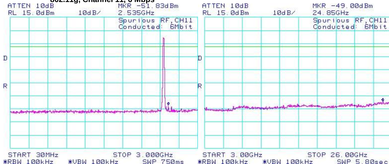
Figure 3-30: Spurious Conducted RF Emissions 802.11g, Channel 11, 6 Mbps
