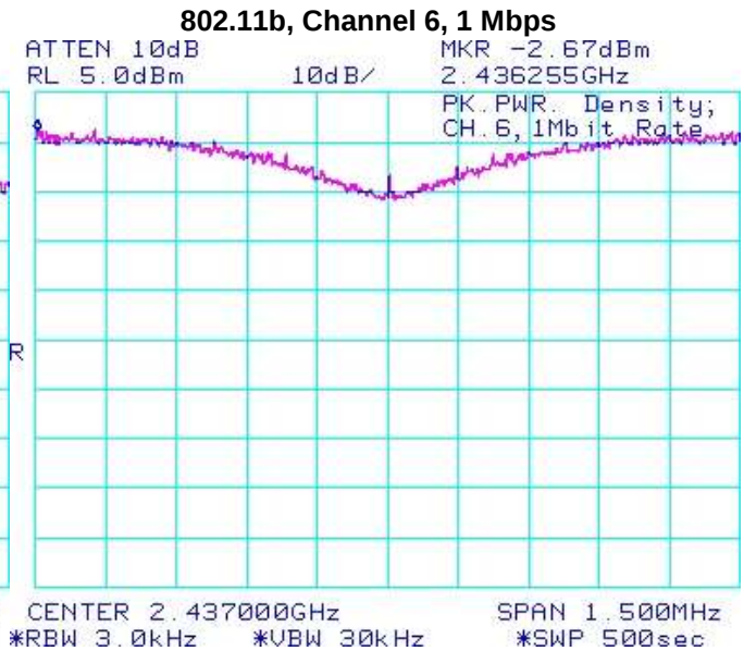
Figure 3-17: Peak Power Spectral Density
