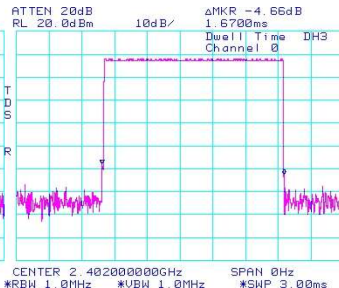
Figure 2-16: Time of Occupancy (Dwell Time) Freq. Hopping, Static PBRS, DH3
