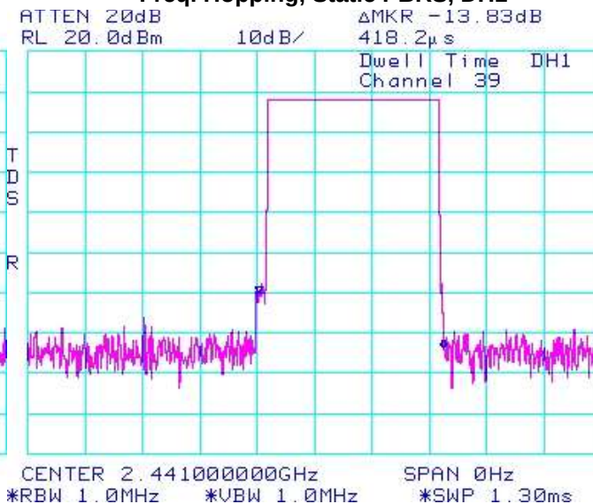
Figure 2-14: Time of Occupancy (Dwell Time)
