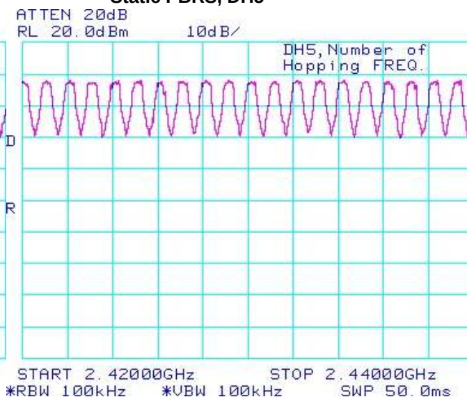
Figure 2-10: Number of Hopping Frequencies Static PBRS, DH5
