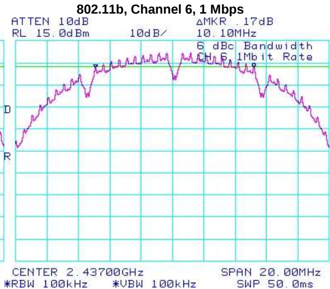
Figure 3-2: 6 dB Bandwidth
