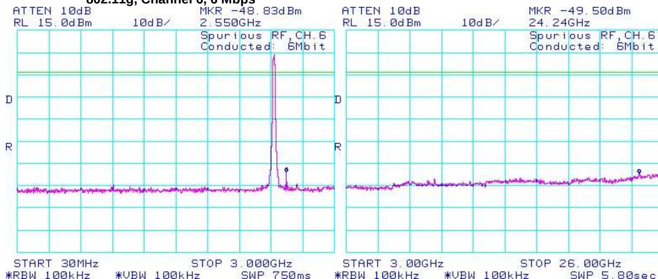
Figure 3-29: Spurious Conducted RF Emissions 802.11g, Channel 6, 6 Mbps
