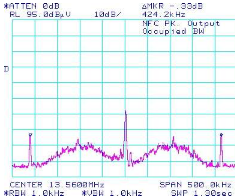
Figure 4-1: Occupied Bandwidth, NFC TX Frequency = 13.56 MHz
