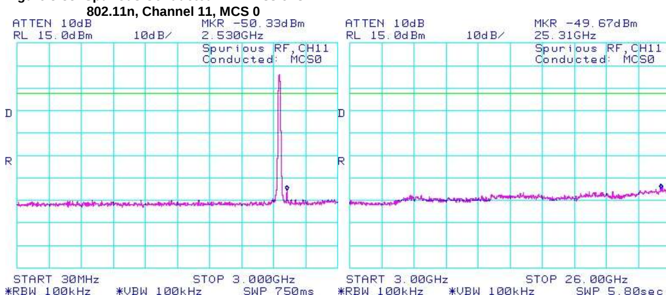
Figure 3-33: Spurious Conducted RF Emissions
