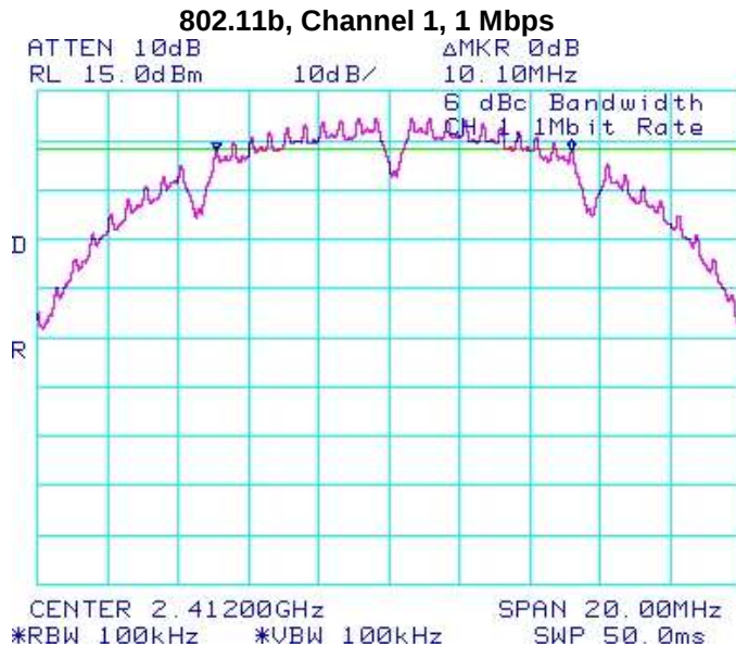
Figure 3-1: 6 dB Bandwidth
