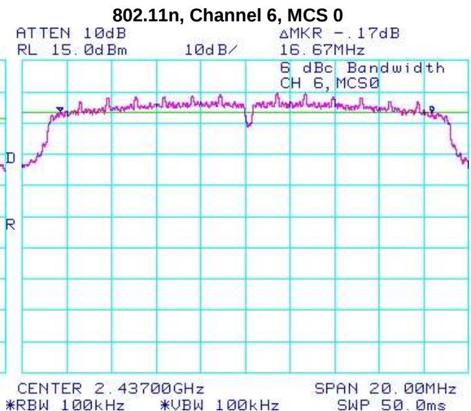
Figure 3-8: 6 dB Bandwidth
