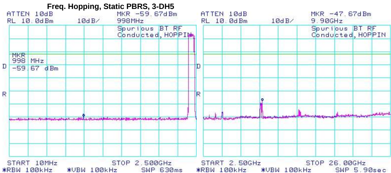
Figure 2-43 : Spurious RF Conducted Emissions
