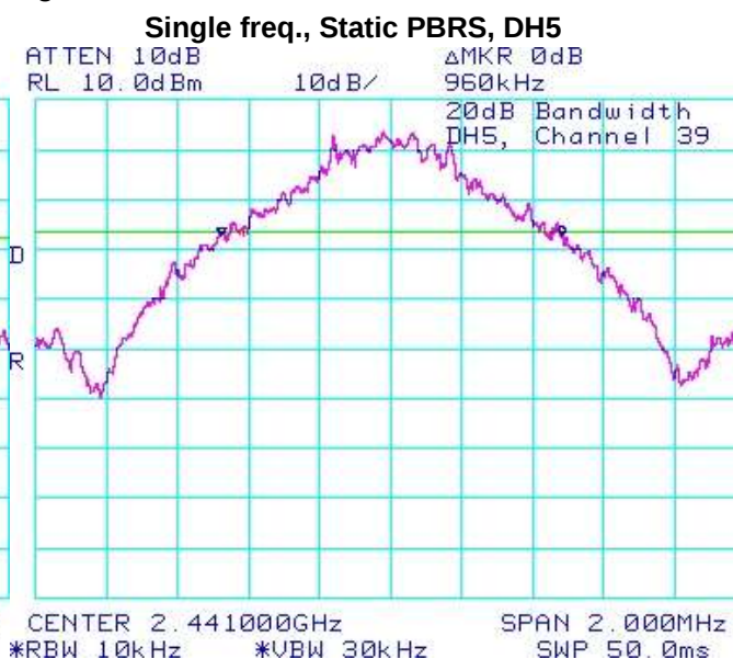
Figure 2-2: 20 dB Bandwidth
