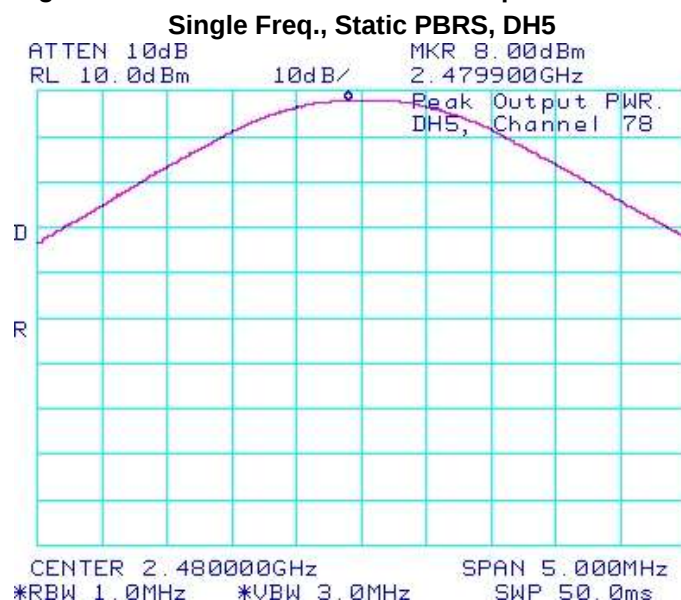
Figure 2-24: Max. Peak Conducted Output Power
