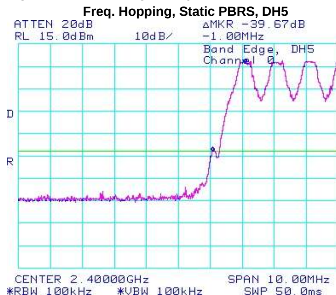
Figure 2-30: Band Edge Compliance
