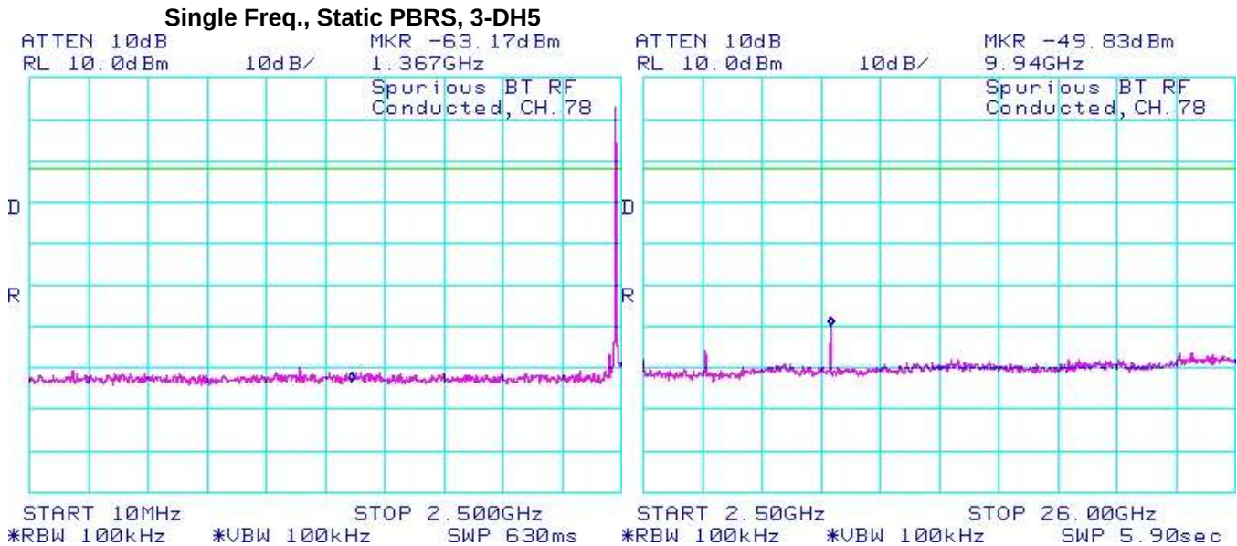
Figure 2-42: Spurious RF Conducted Emissions
