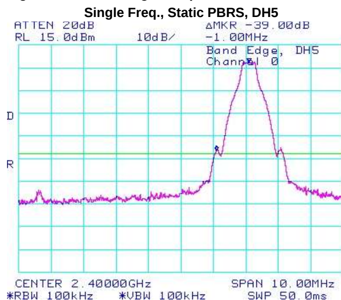
Figure 2-28: Band Edge Compliance
