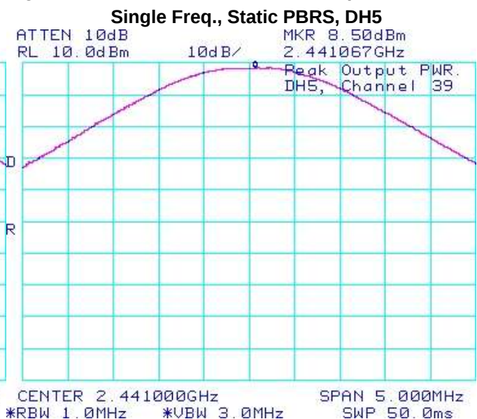
Figure 2-23: Max. Peak Conducted Output Power
