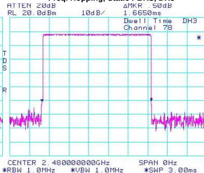
Figure 2-18 : Time of Occupancy (Dwell Time) Freq. Hopping, Static PBRS, DH3
