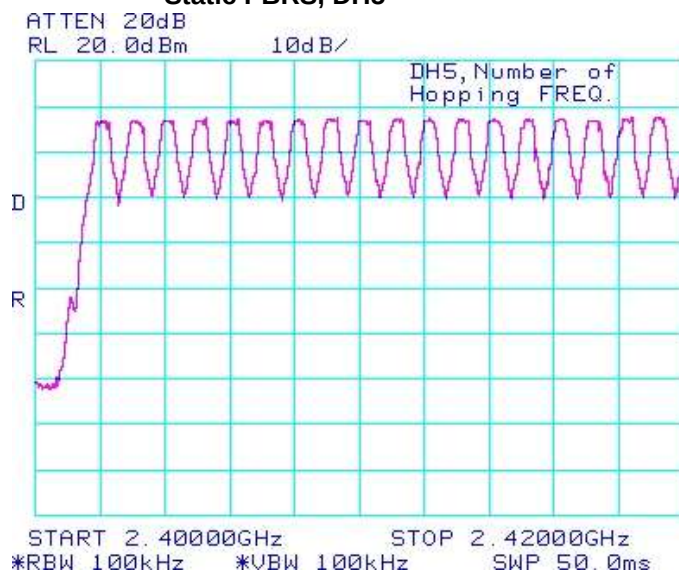
Figure 2-9: Number of Hopping Frequencies Static PBRS, DH5
