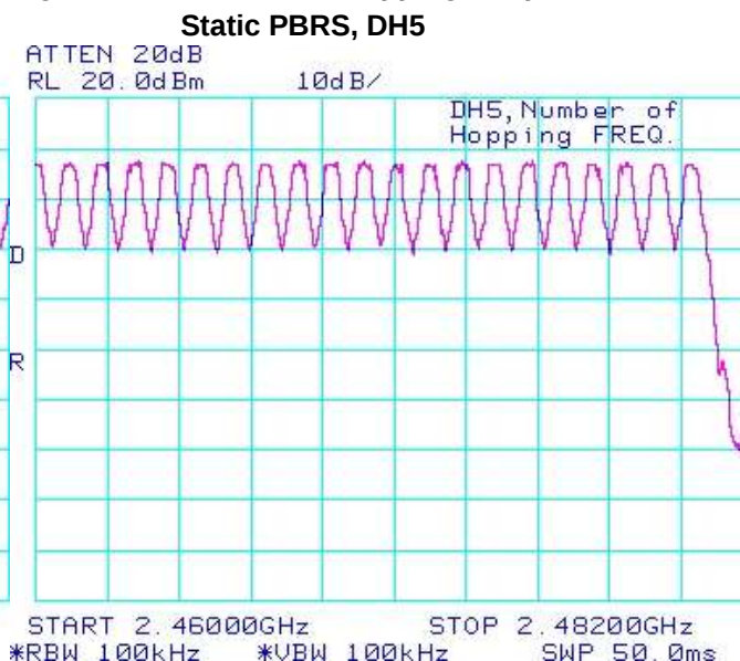
Figure 2-12: Number of Hopping Frequencies
