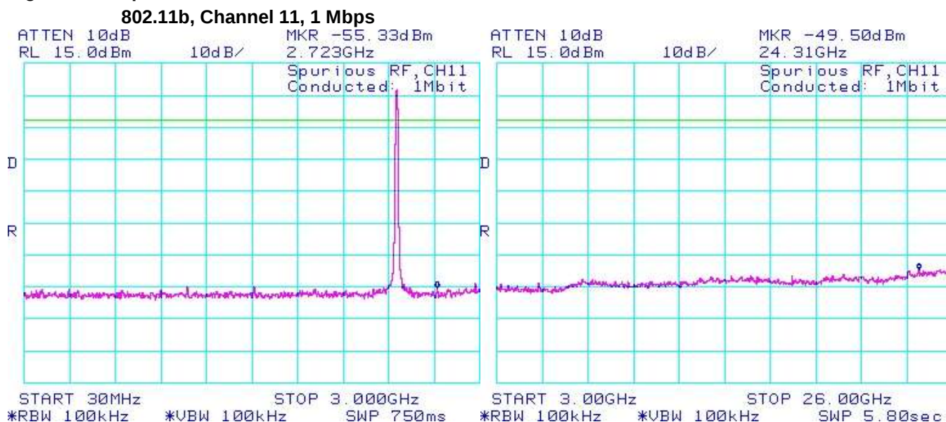
Figure 3-27: Spurious Conducted RF Emissions
