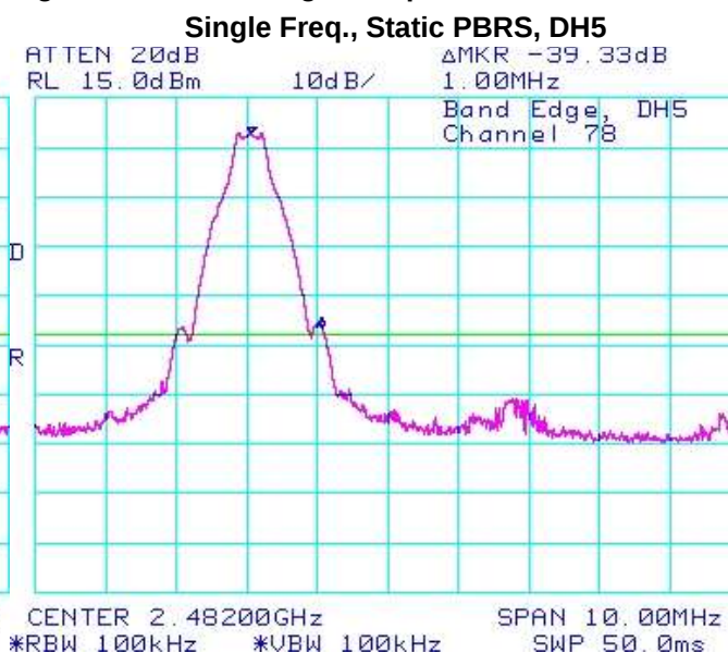
Figure 2-29: Band Edge Compliance
