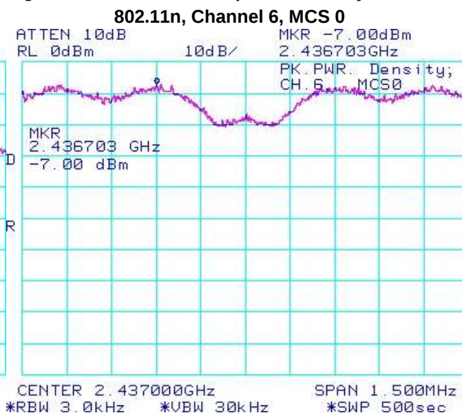
Figure 3-23: Peak Power Spectral Density
