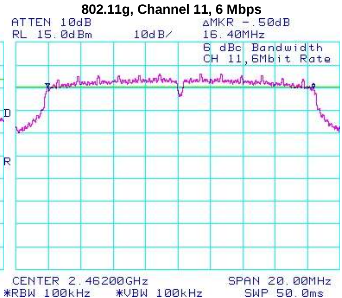
Figure 3-6: 6 dB Bandwidth
