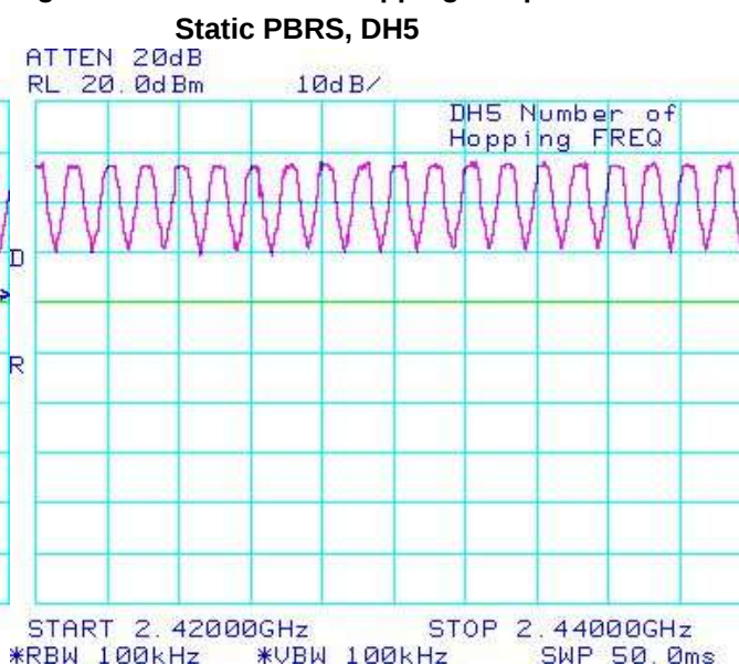
Figure 4-10: Number of Hopping Frequencies
