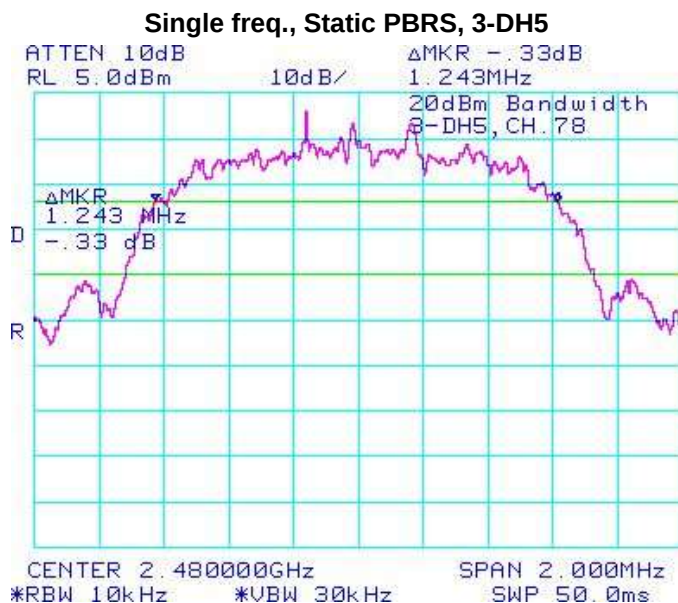
Figure 4-6: 20 dB Bandwidth
