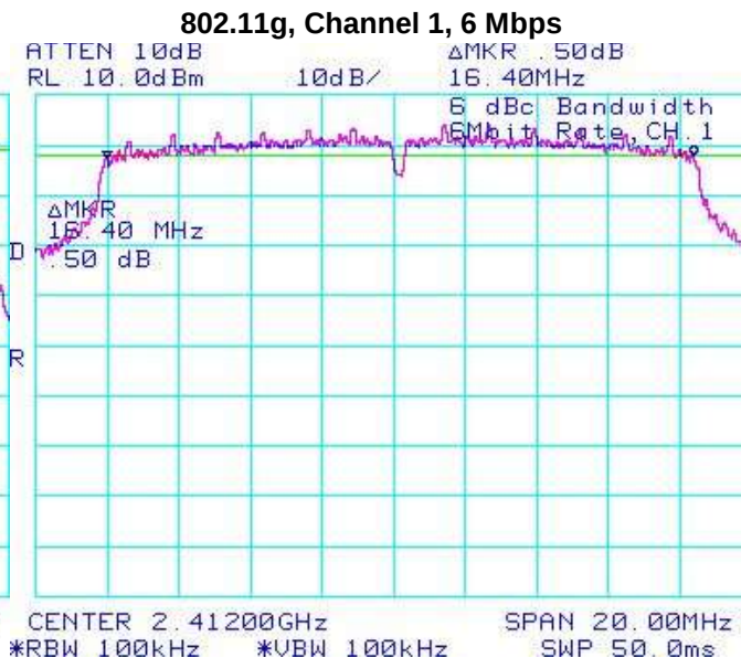
Figure 5-4: 6 dB Bandwidth
