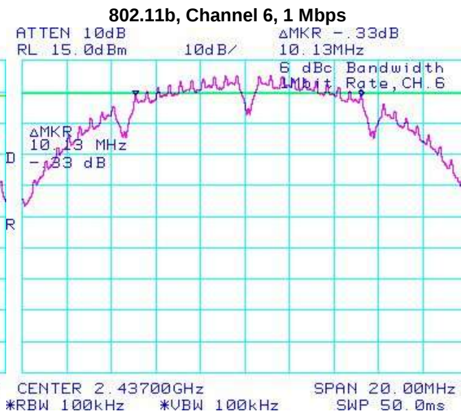
Figure 5-2: 6 dB Bandwidth
