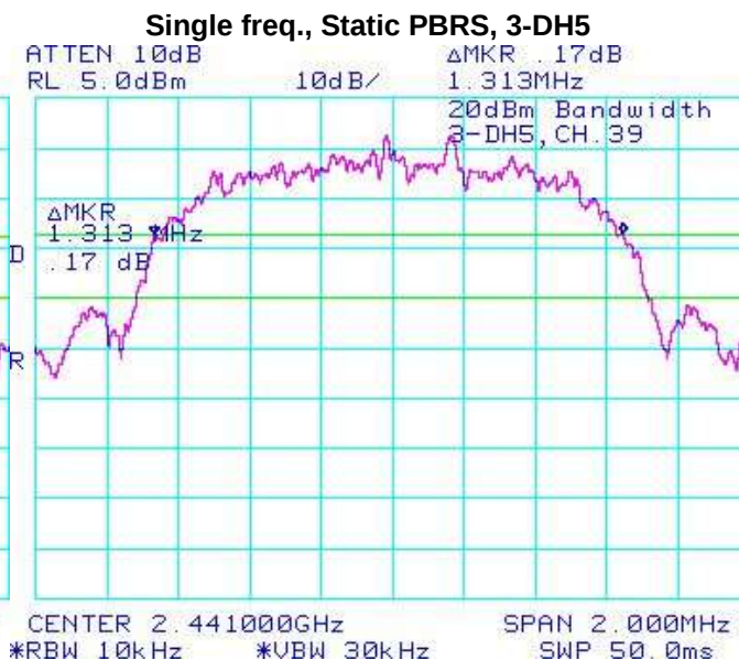
Figure 4-5: 20 dB Bandwidth
