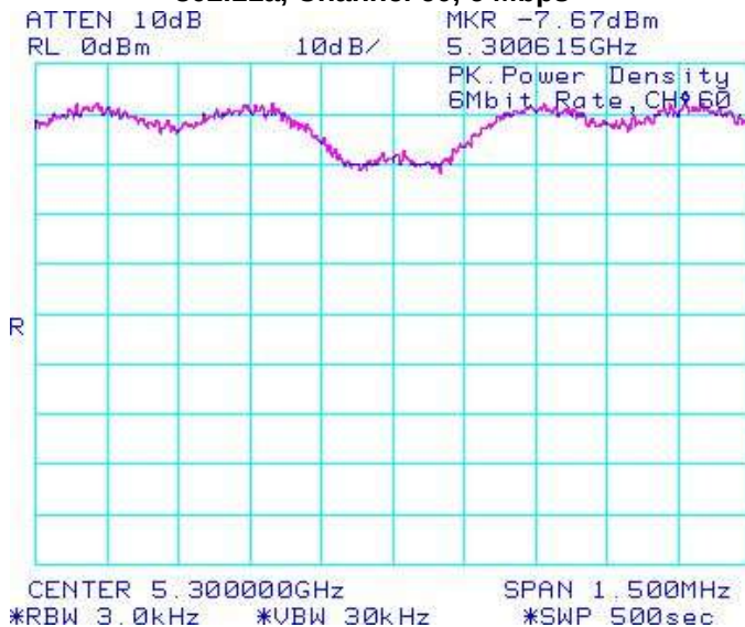
Figure 6-22: Peak Power Spectral Density 802.11a, Channel 60, 6 Mbps
