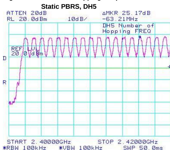
Figure 4-9: Number of Hopping Frequencies
