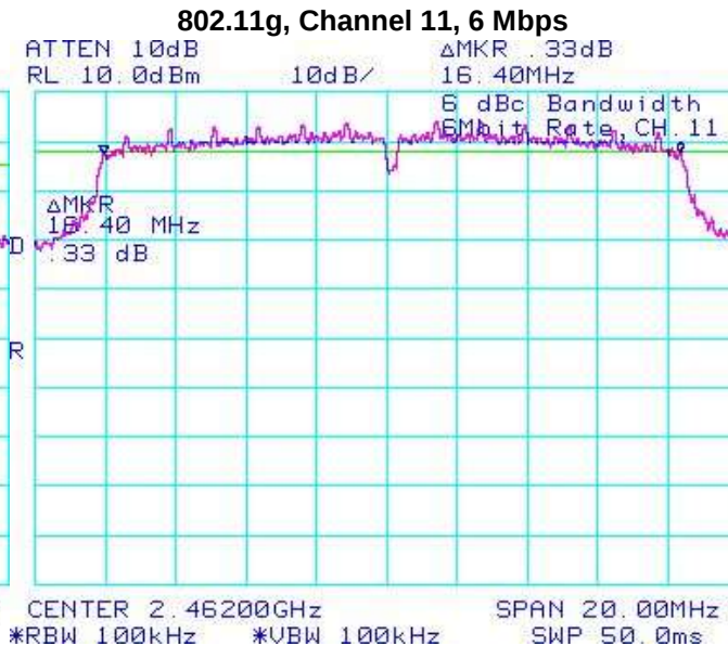
Figure 5-6: 6 dB Bandwidth
