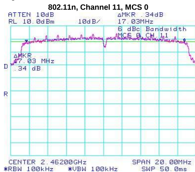
Figure 5-9: 6 dB Bandwidth
