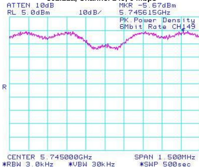
Figure 6-24: Peak Power Spectral Density 802.11a, Channel 149, 6 Mbps
