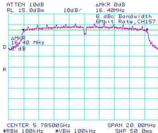
Figure 6-10: 6 dB Bandwidth
