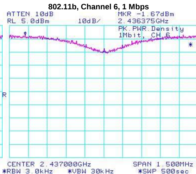
Figure 5-17: Peak Power Spectral Density
