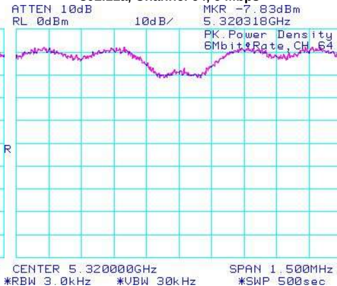
Figure 6-23: Peak Power Spectral Density 802.11a, Channel 64, 6 Mbps
