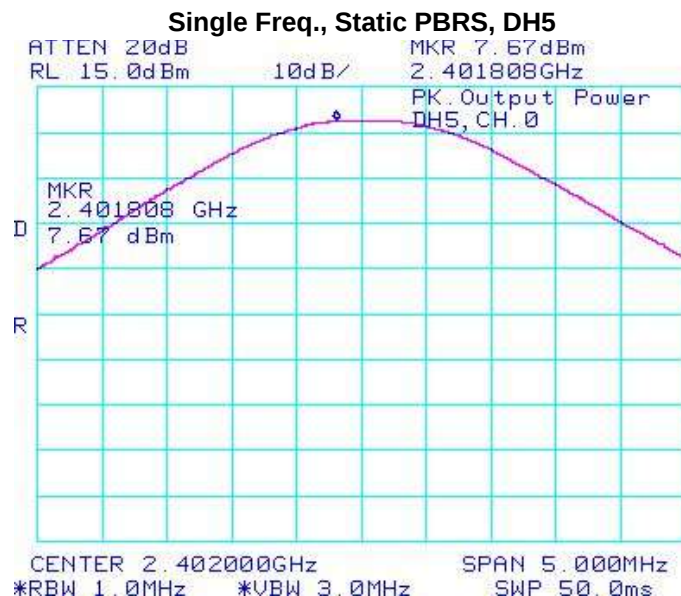
Figure 4-22: Max. Peak Conducted Output Power
