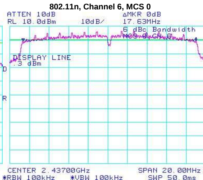
Figure 5-8: 6 dB Bandwidth
