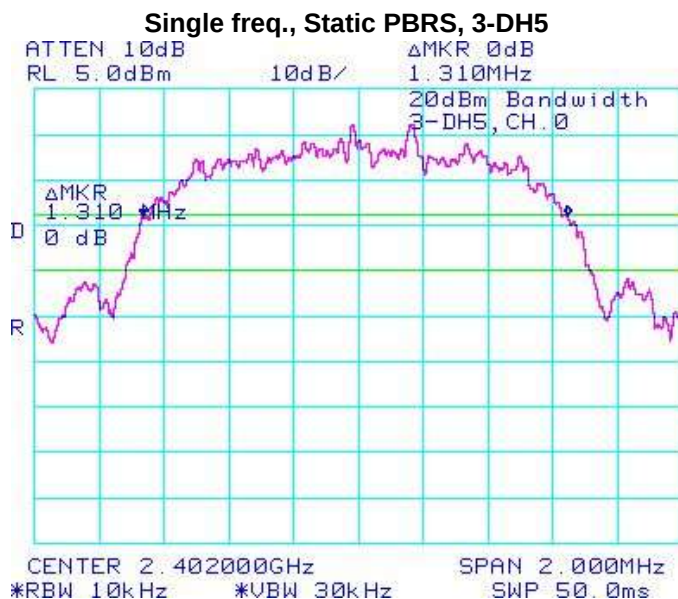
Figure 4-4: 20 dB Bandwidth
