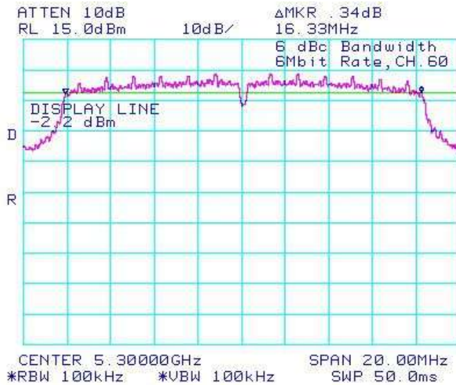
Figure 6-5: 6 dB Bandwidth
