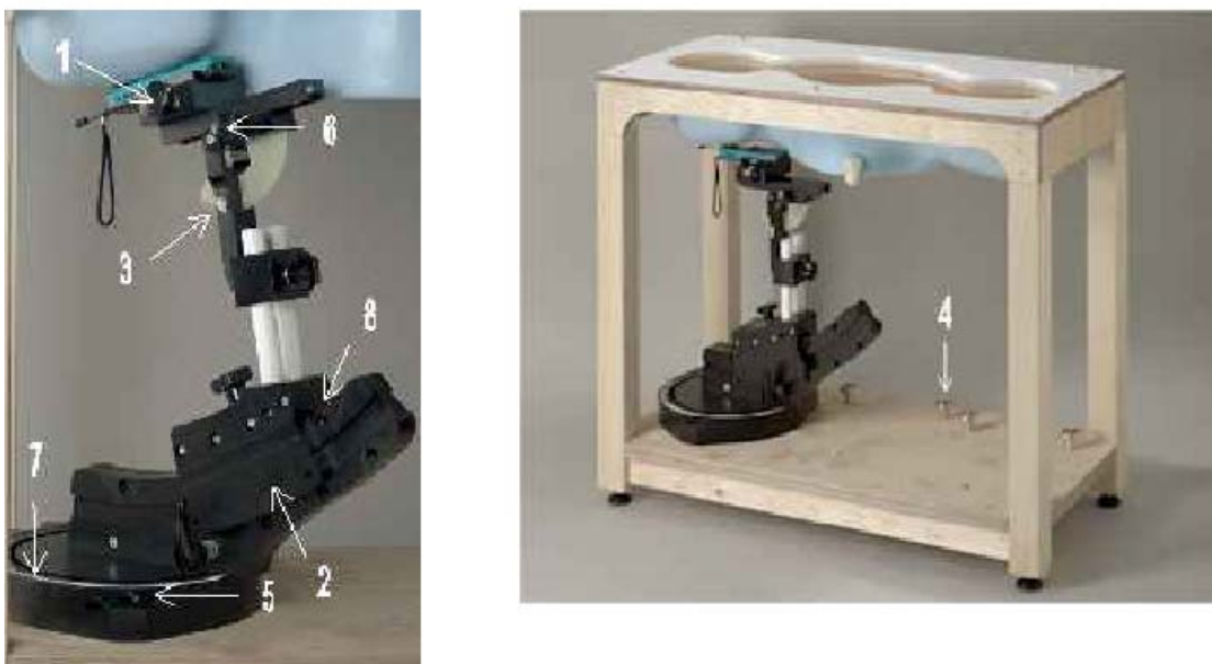
Figure 8.1.1. Device Holder
