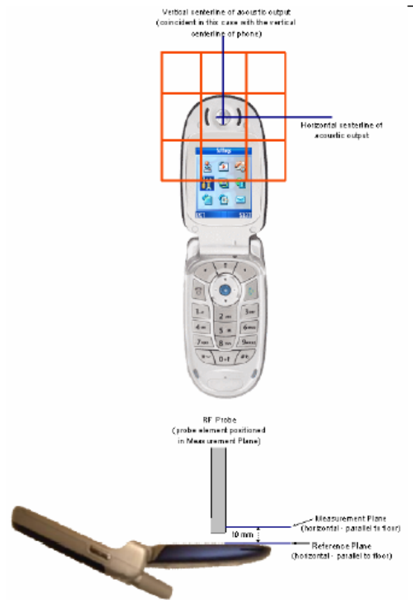
Figure 5.3: WD reference plane for RF emission measurements Figure 5.4: HAC Phantom/Test Arch
