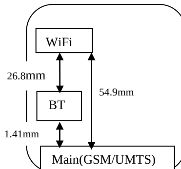
Figure 1.9.2. Back view of device showing closet distance between antenna pairs
