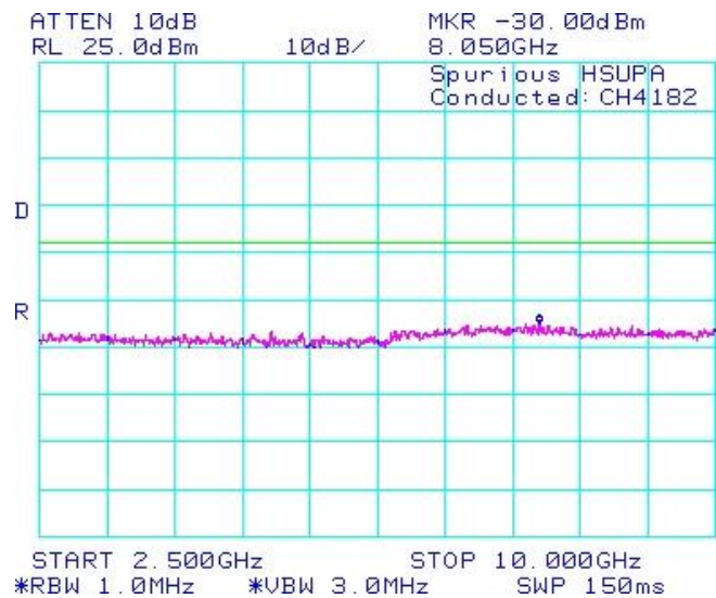
Figure 1-26b: Band 5 , Spurious Conducted Emissions, Middle channel
