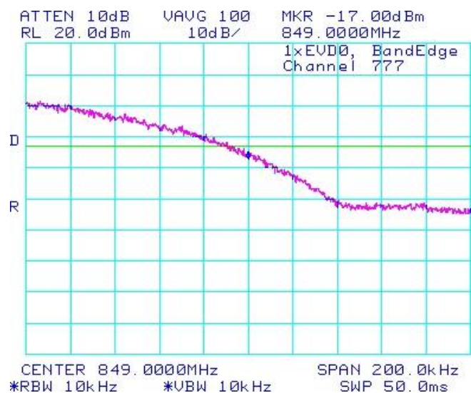
Figure 1-41b: Cellular , High Channel Mask
