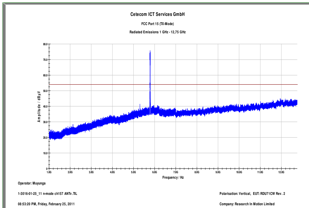
Plot 70: 1 GHz to 12.75 GHz / channel 157 (vertical), n-mode
