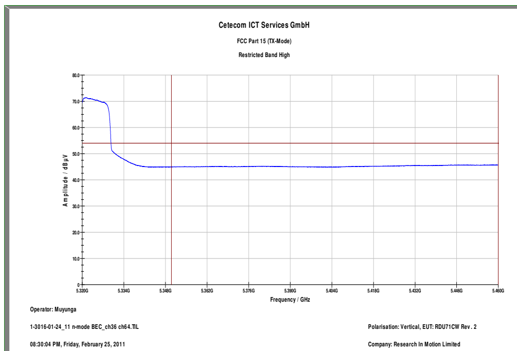
Plot 5: 5350 MHz / n-mode (radiated)
