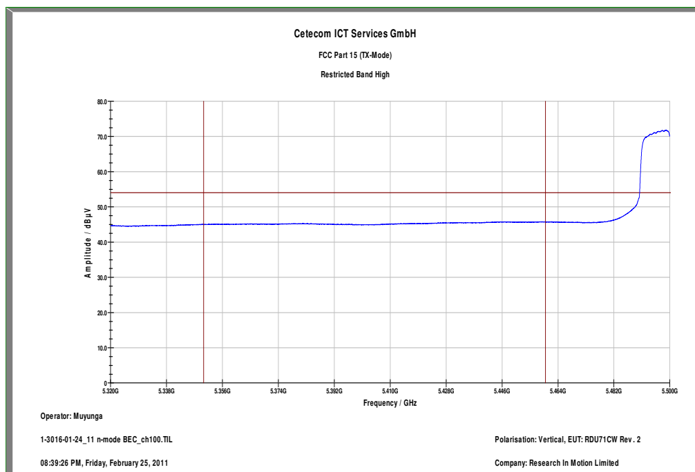
Plot 6: 5470 MHz / n-mode (radiated)
