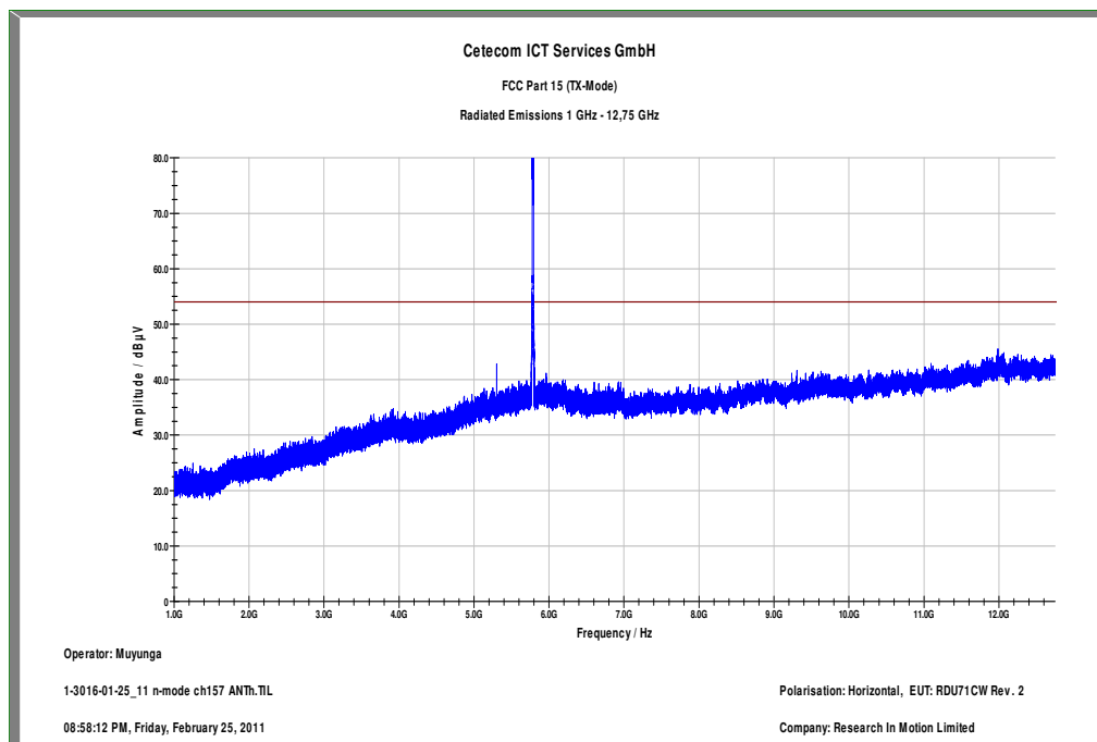
Plot 71: 1 GHz to 12.75 GHz / channel 157 (horizontal), n-mode
