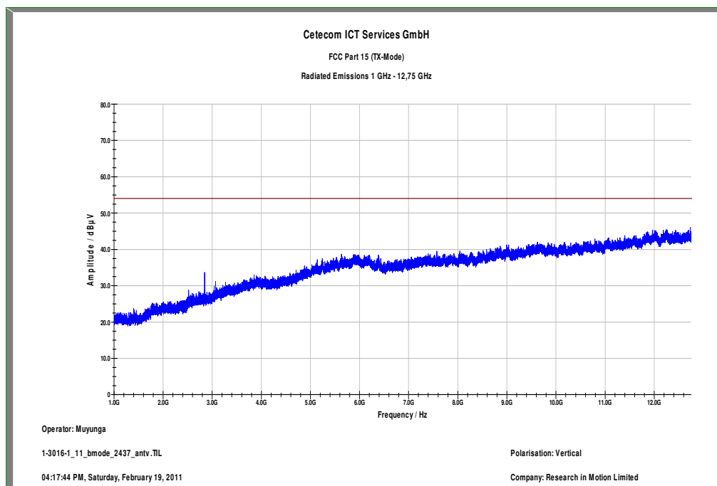
Plot 7: 1 GHz to 12.75 GHz / channel 06 (vertical), b-mode
