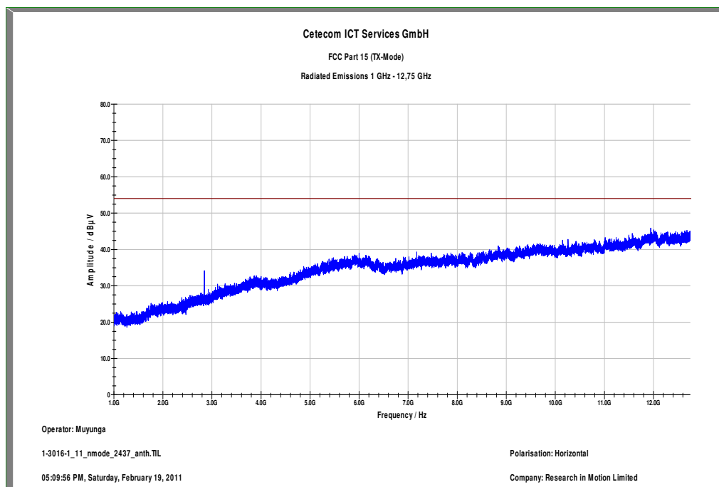
Plot 23: 1 GHz to 12.75 GHz / channel 06 (horizontal), n-mode
