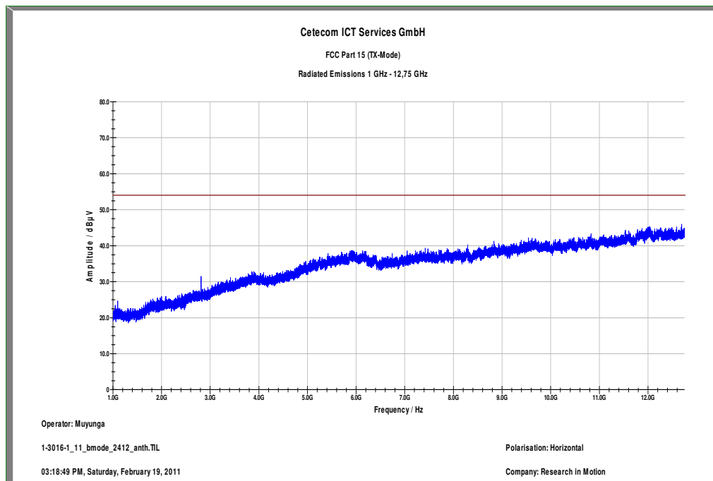
Plot 3: 1 GHz to 12.75 GHz / channel 01 (horizontal), b-mode
