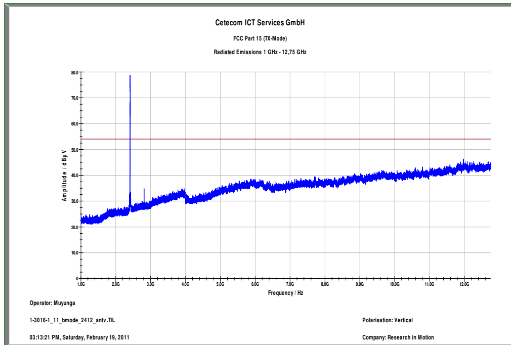
Plot 2: 1 GHz to 12.75 GHz / channel 01 (vertical), b-mode
