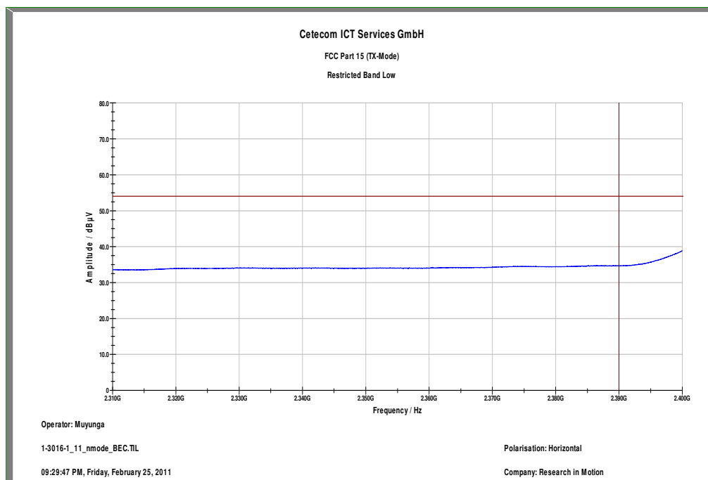
Plot 5: Lower Restricted Band / n-mode (radiated)
