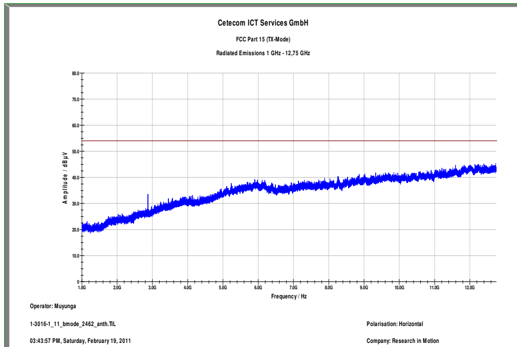
Plot 13: 1 GHz to 12.75 GHz / channel 11 (horizontal), b-mode
