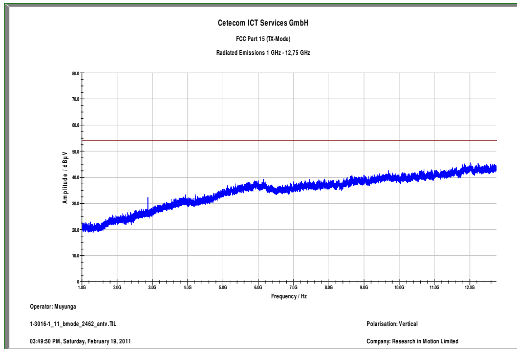
Plot 12: 1 GHz to 12.75 GHz / channel 11 (vertical), b-mode
