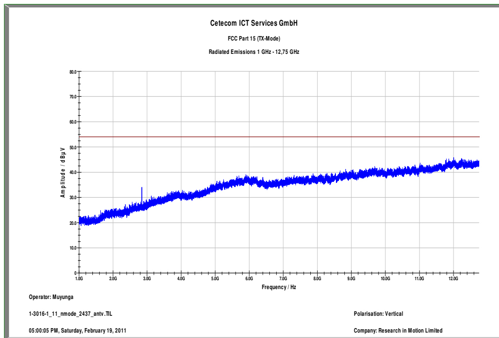
Plot 22: 1 GHz to 12.75 GHz / channel 06 (vertical), n-mode
