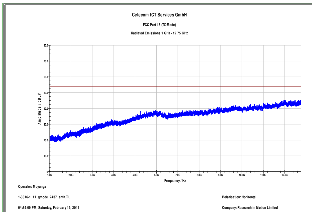
Plot 18: 1 GHz to 12.75 GHz / channel 06 (horizontal), g-mode
