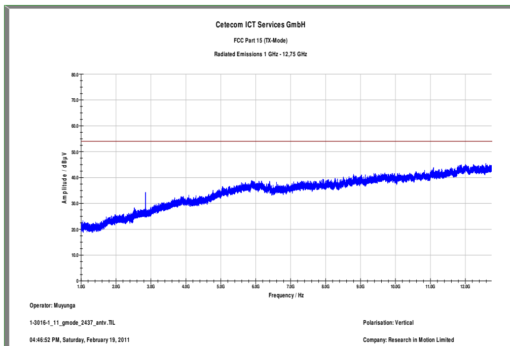
Plot 17: 1 GHz to 12.75 GHz / channel 06 (vertical), g-mode
