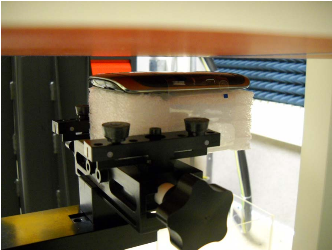
Photo 2. Rear 10mm
