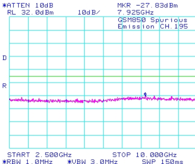
Figure 1-42a: GSM850 band, Spurious Conducted Emissions, Middle channel in Edge Mode
