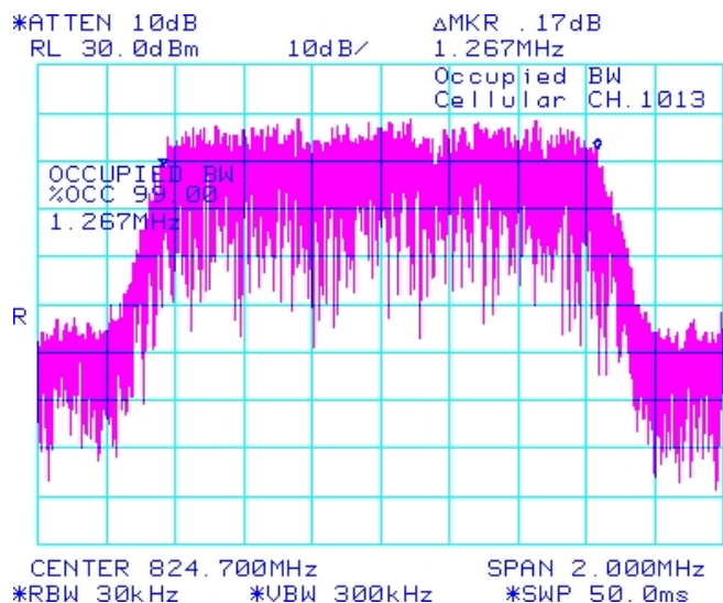
Figure 1-13b: Occupied Bandwidth, Cellular Low Channel
