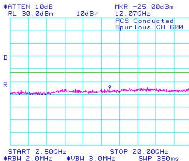
Figure 1-10b: PCS, Spurious Conducted Emissions, Middle Channel
