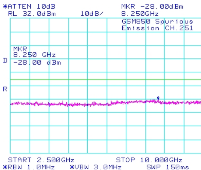
Figure 1-44a: GSM850 band, Spurious Conducted Emissions, High channel in Edge Mode
