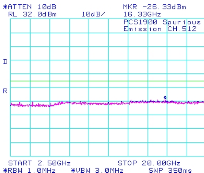
Figure 1-46a: PCS1900 band, Spurious Conducted Emissions, Low channel in Edge Mode
