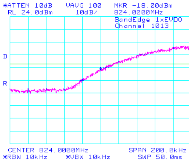
Figure 1-41b: Cellular , Low Channel Mask
