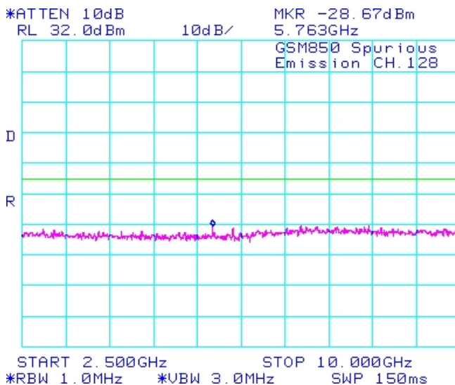
Figure 1-40a: GSM850 band, Spurious Conducted Emissions, Low channel in Edge Mode
