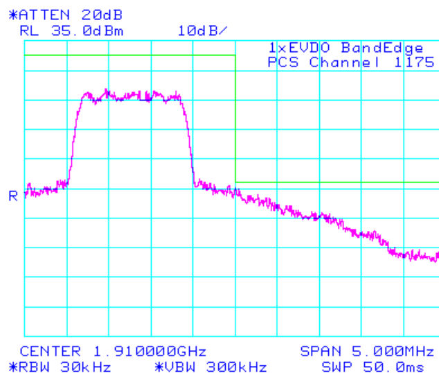
Figure 1-45b: PCS , High Channel Mask
