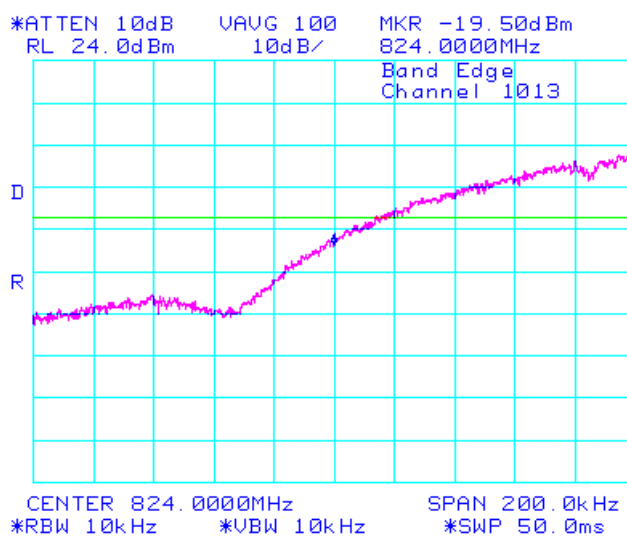
Figure 1-20b: Cellular Low Channel Mask
