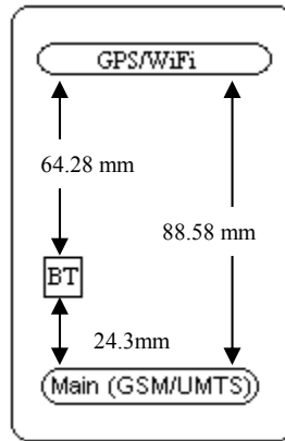
Figure 1.9.1. Back view of device showing closest distance between antenna pairs
