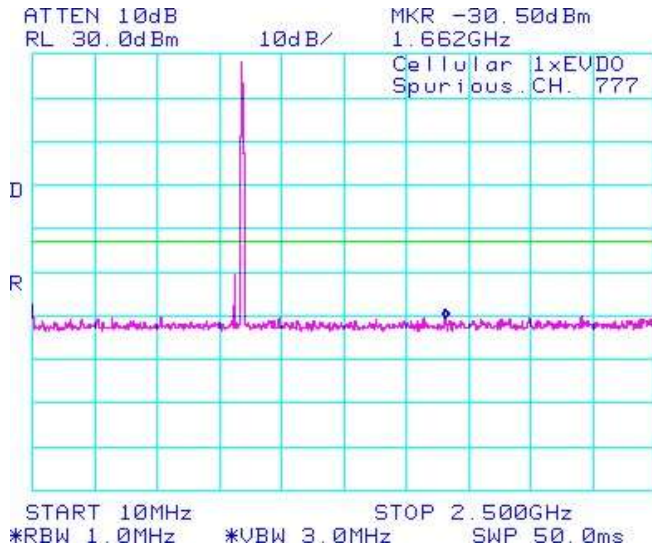
Figure 1-27b: Cellular , Spurious Conducted Emissions, High Channel
