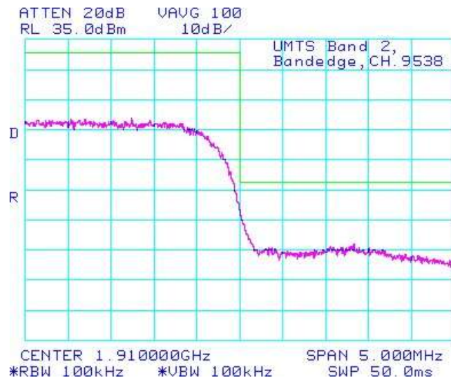
Figure 1-22c: BAND 2 High Channel Mask
