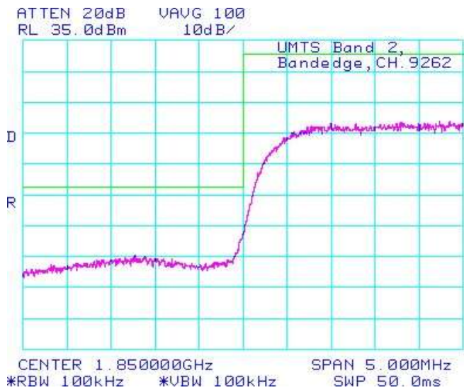
Figure 1-21c: BAND 2 Low Channel Mask
