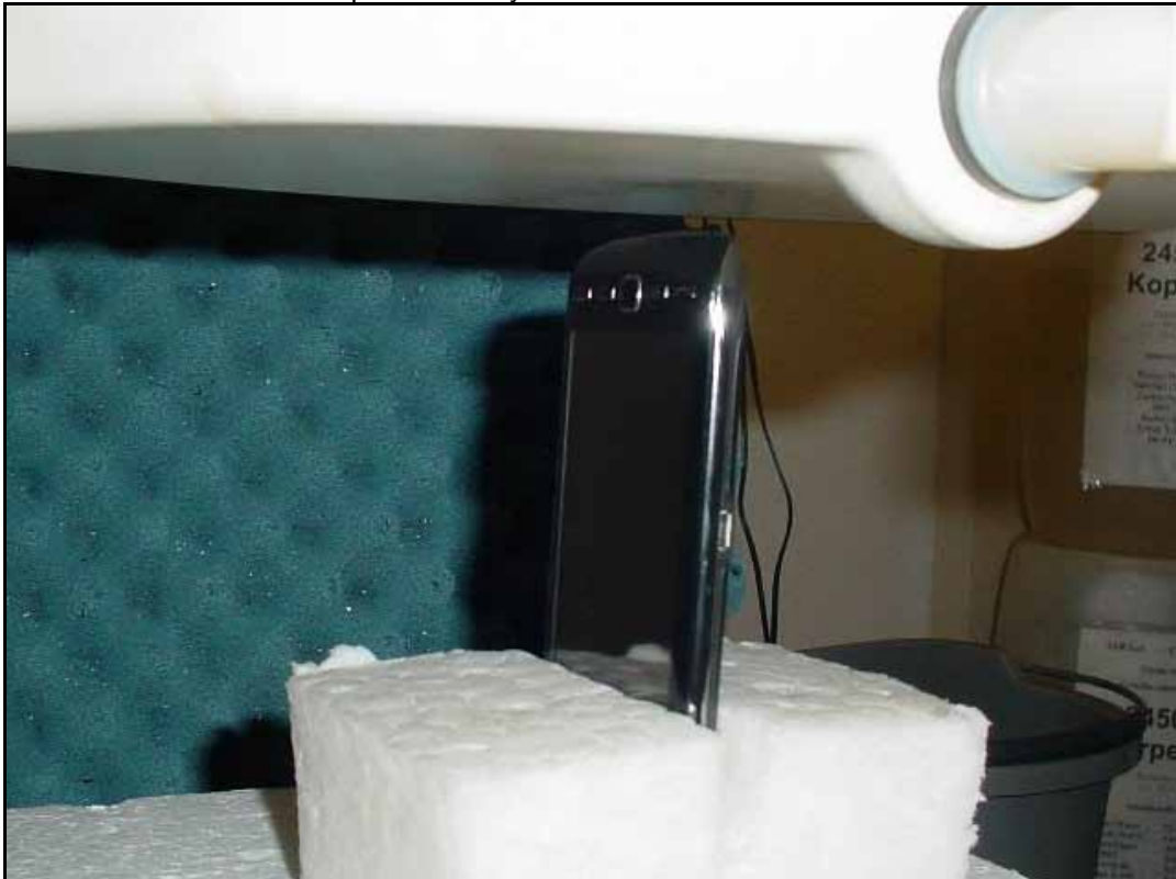
Photo 14: Test position body worn top side with 10 mm distance
