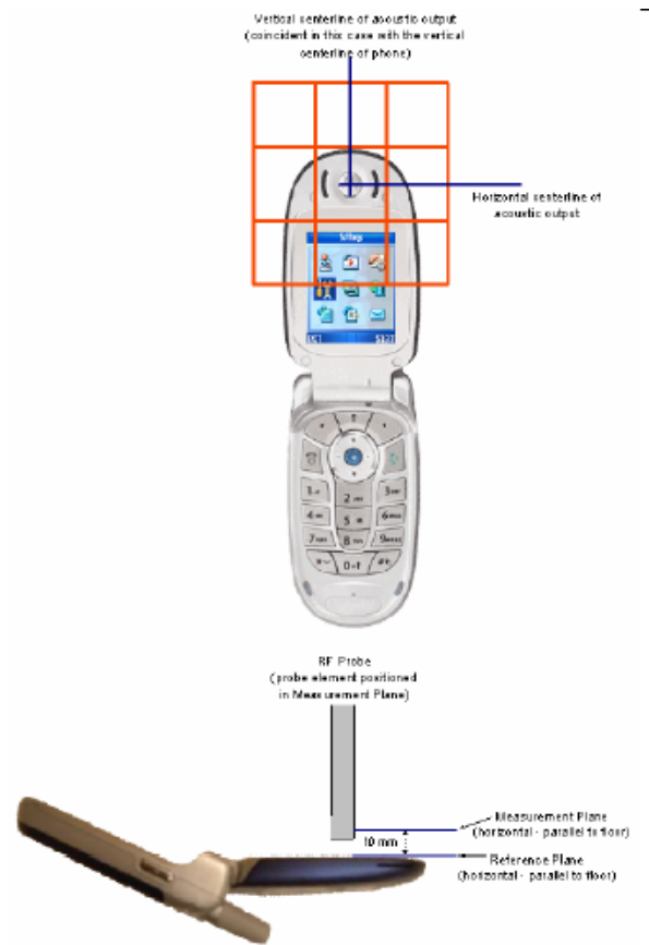
Figure 4: WD reference plane for RF emission measurements Figure 5: HAC Phantom/Test Arch
